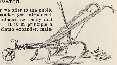
"Iron Age" No. 6 Horse Hoe and Cultivator with Seven-Tooth or Furrow-Closing Attachment.
