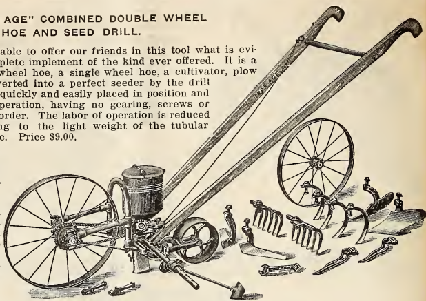
The "Iron Age" Combined Double Wheel Hoe and Seed Drill. $9.00.
