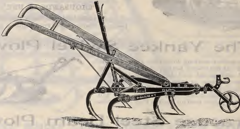
No. 123—Expanding Lever, five 3-inch Points, Wing Points, Shovel Point and Stationary Wheel Price $5.00.
