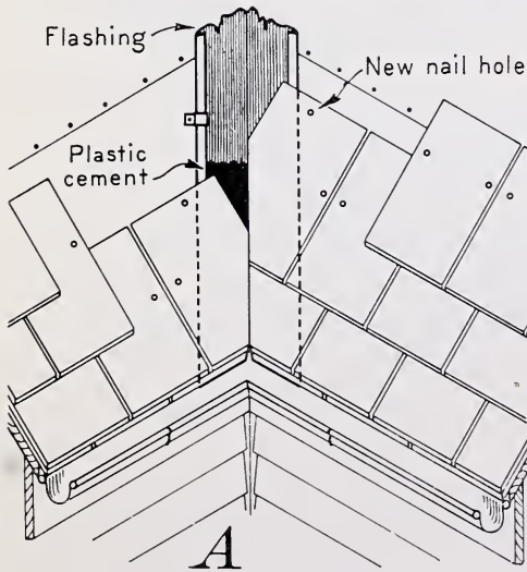
Figure 15.—Flashing in closed valley: A , Long metal strip under shingles; B , short pieces of metal intermembered with shingles.
