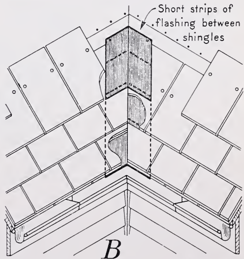
Figure 15.—Flashing in closed valley: A , Long metal strip under shingles; B , short pieces of metal intermembered with shingles.
