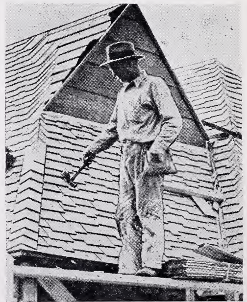
Figure 2.—Finishing hips and ridges "Boston" style.
