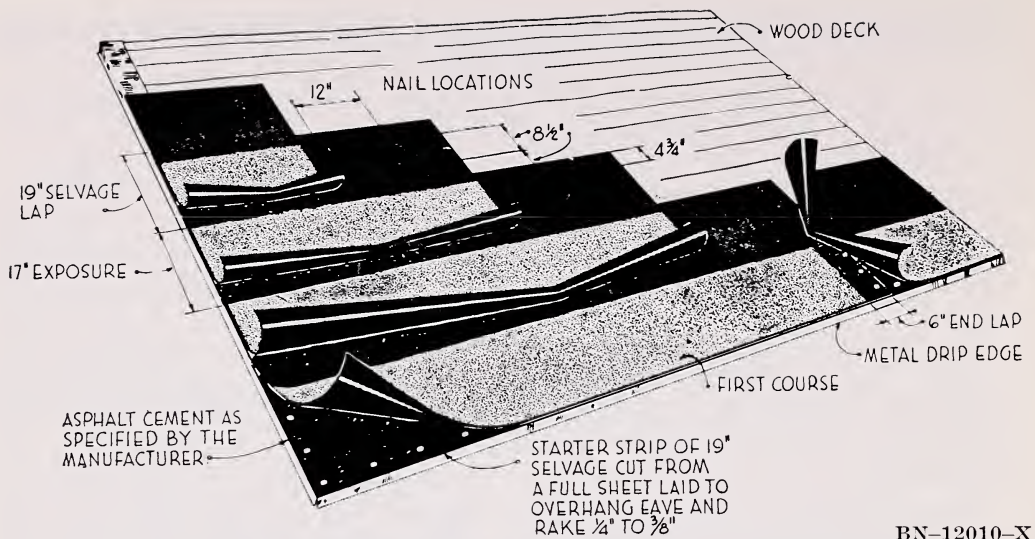
Figure 6.—Installation of selvage-edge roll roofing.
