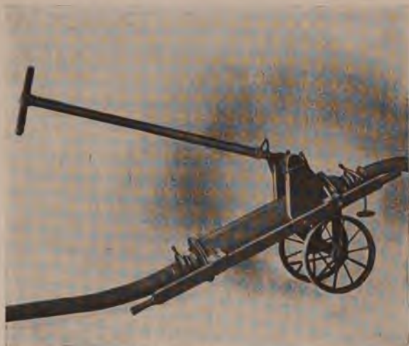
Fig. 31.—Hand-pump for use with "odorless excavator" apparatus.
