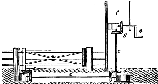
[Fig. 62. Plan for opening the gate from the interior of the Lodge.]
