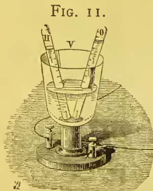
Gaiffe's voltameter for collecting the gasses separately, H and O.
