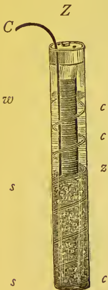
FIG. 102. MAYER AND MELTZER'S SULPHATE OF COPPER BATTERY.
