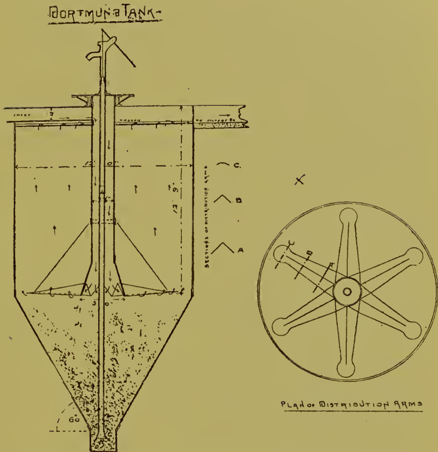
FIG. 18. SECTION AND PLAN OF DORTMUND PRECIPITATING TANK.
