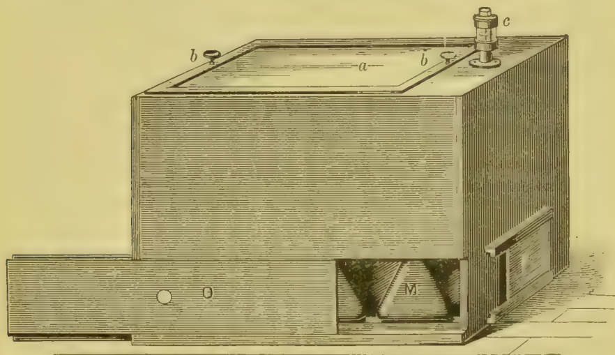
FIG. 66.—Modified Auvarde incubator or couveuse : a , glass plate of the movable lid ( b ); c , ventilating tube containing small rotary fan; κ , ventilating slide; M , hot-water cans; o , slide closing hot-air chamber.
