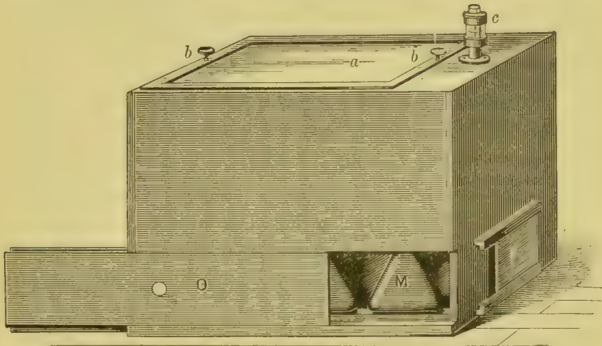
FIG. 66.—Modified Auvard incubator or couveuse : a , glass plate of the movable lid ( b ); c , ventilating tube containing small rotary fan; k , ventilating slide; m , hot-water cans; o , slide closing hot-air chamber.
