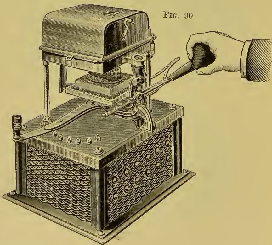
HAMMOND ELECTRIC FURNACE NO. 4, CLOSED AND OPEN
