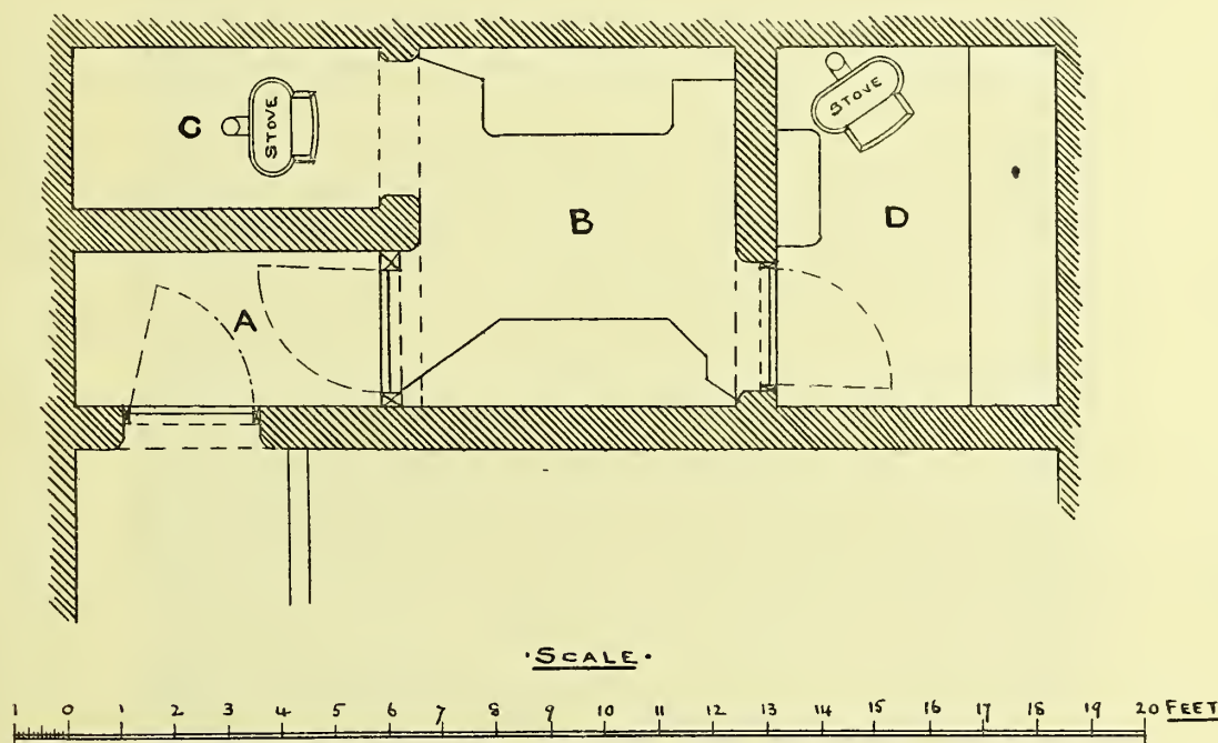
FIG. 4.—PLAN OF INCUBATING CHAMBER.
