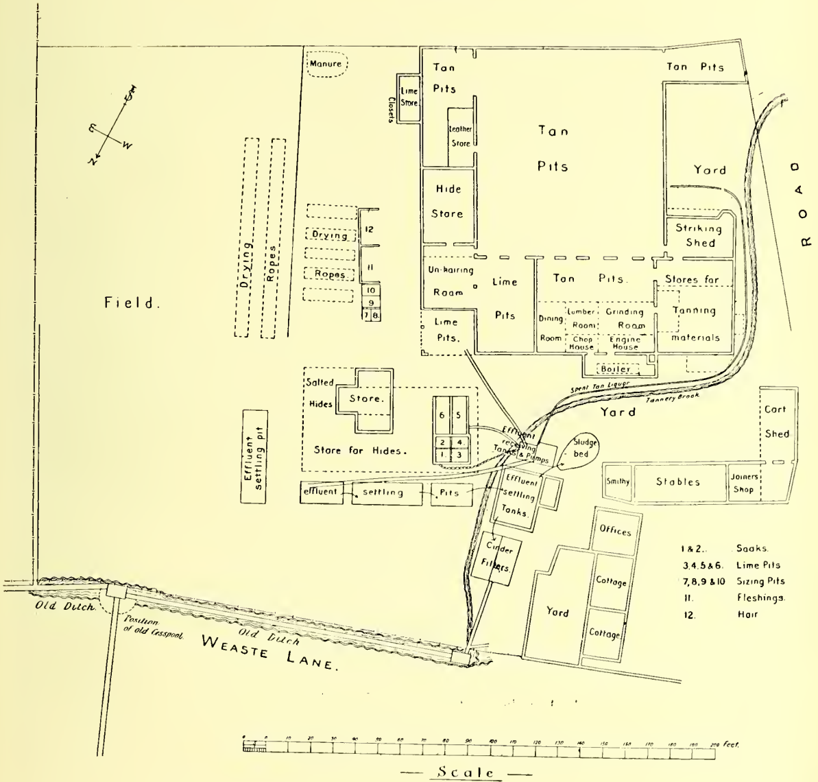
PLAN OF THE TANNERY.
