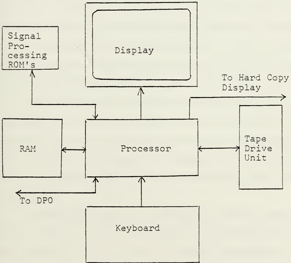
Figure 25. Block Diagram of System Controller Hardware
