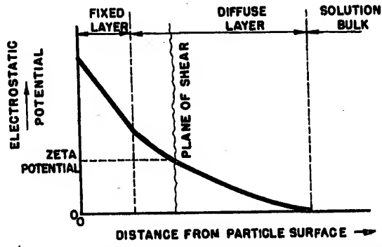
Fig. 7 - Potentials Through the Electrostatic Field Surrounding a Charged Hydrophilic Colloid Particle. (From Rich, p. 138.)
