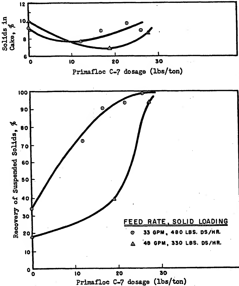
Fig. 33 - Performance of 24 x 60 Inch Centrifuge Dewatering Waste Sludge, St. Petersburg, Fla.
