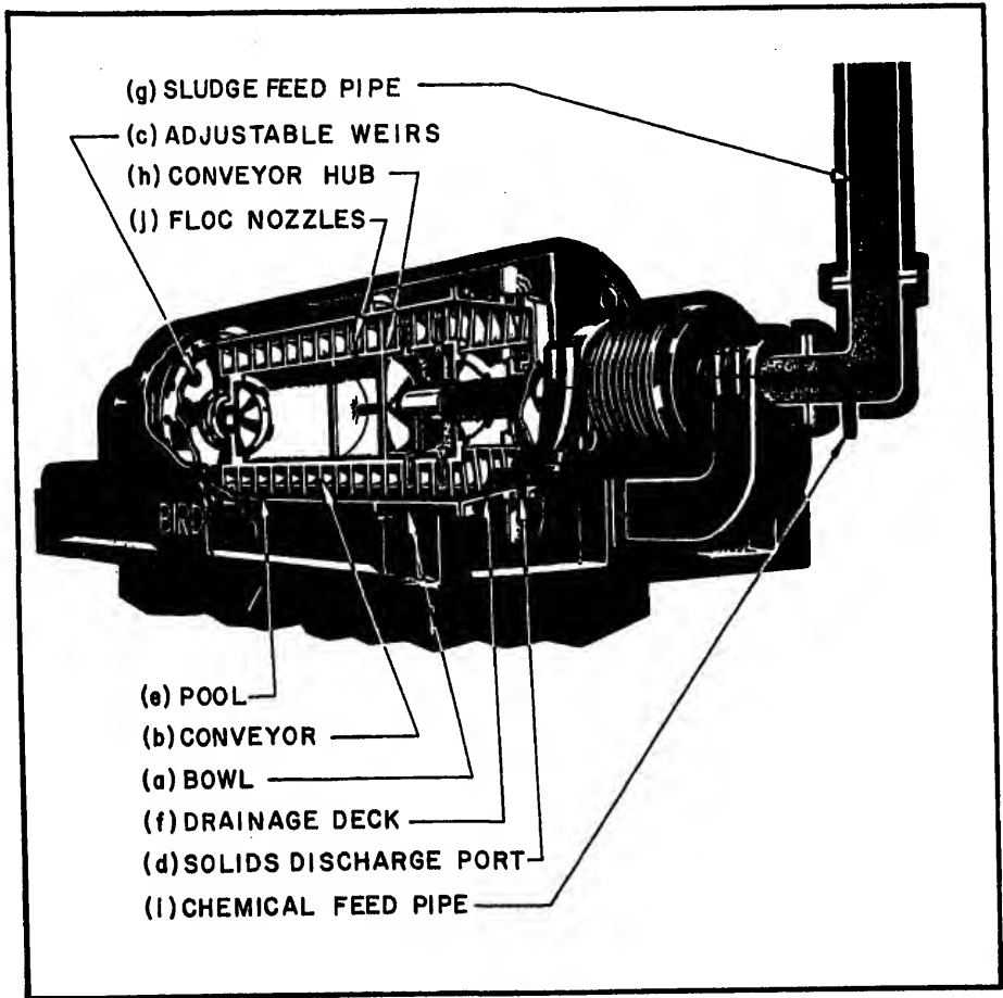
Fig. 8 - Bird Solid Bowl Continuous Centrifuge With Countercurrent Flow.
