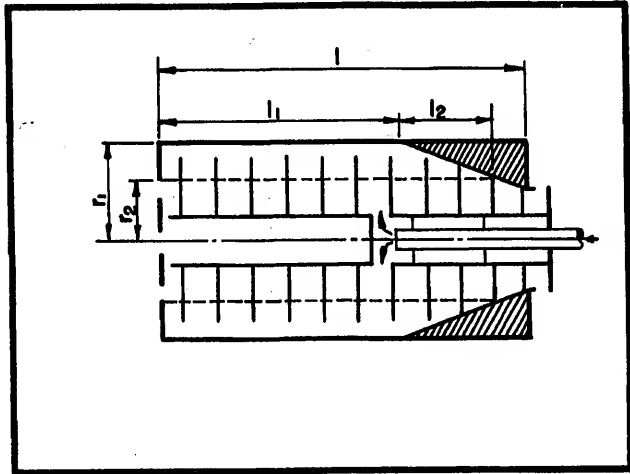
Fig. 4 - Cross-Sectional View of Typical Cylindrical-Type Solid Bowl Centrifuge.
