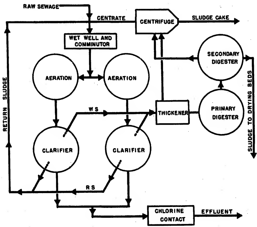
Fig. 13 - Schematic Flow Diagram of the Northeast Sewage Treatment Plant, St. Petersburg, Fla.
