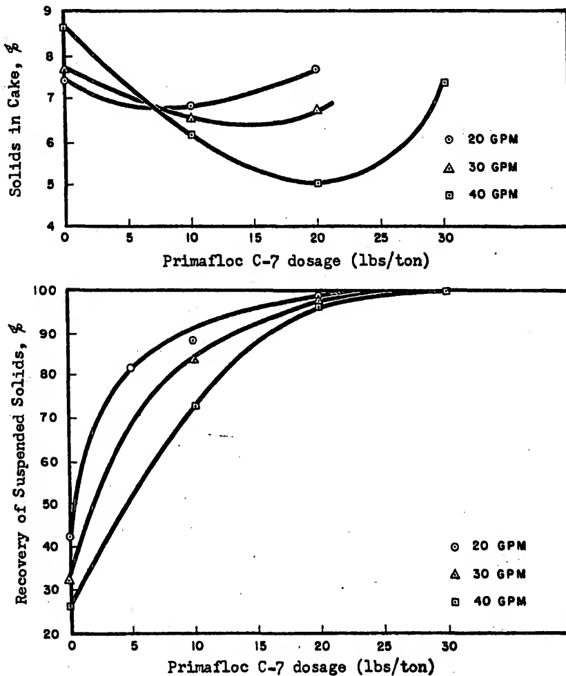
Fig. 30 - Effect of Feed Rate and Polymer Dosage on Performance of 24 x 38 Inch Centrifuge Return Sludge, Treasure Island, Fla.
