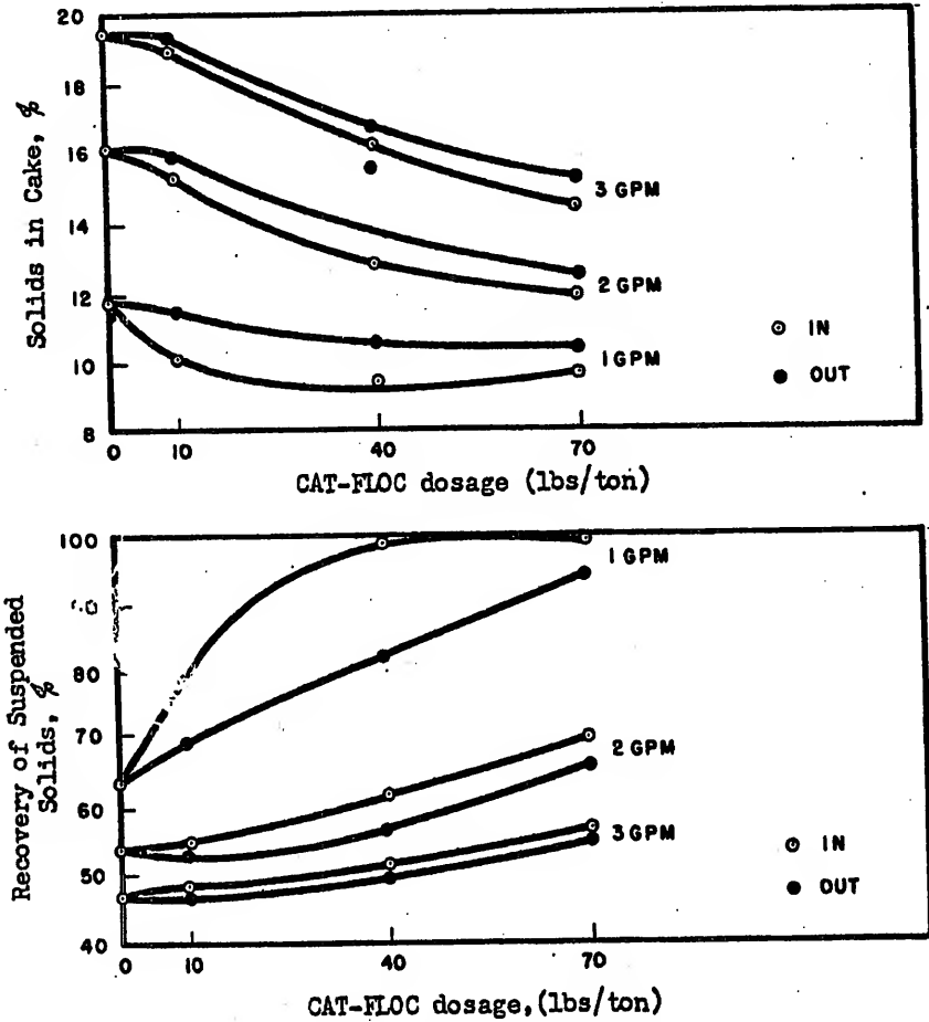
Fig. 15 - Effect of Sludge Feed Rate, Polymer Dosage, and Location Polymer Added on Performance of 6x12 Inch Centrifuge Dewatering Digested Sludge, University of Florida.
