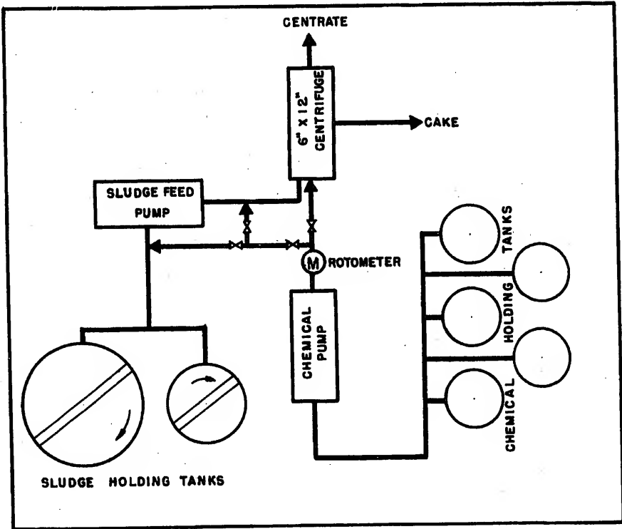
Fig. 10 - Schematic Flow Diagram of Sludge Dewatering Pilot Plant, University of Florida.
