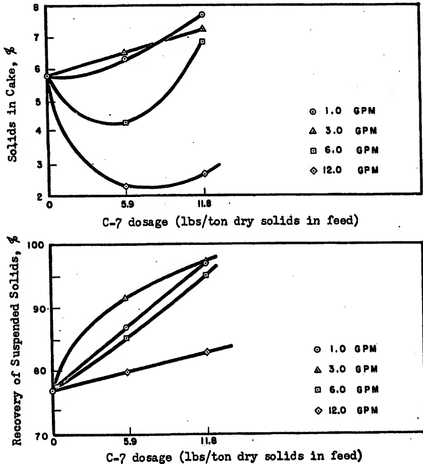
Fig. 34 - Effect of Polymer Dosage and Polymer Dosing Rate on Performance of 24 x 60 Inch Centrifuge Dewatering Return Activated Sludge, St. Petersburg, Fla.
