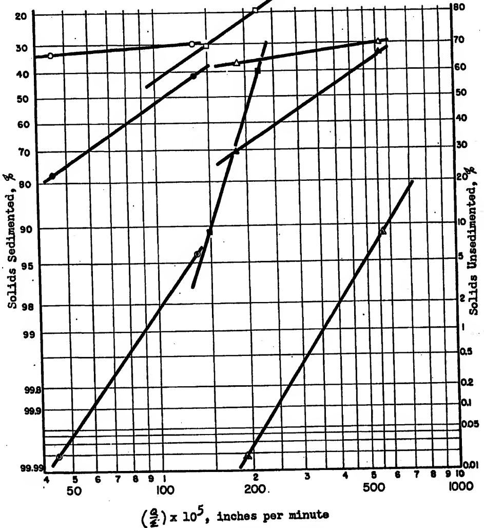
Fig. 41- Sedimentation Performance Versus Parameter \frac{M/D}{\text{min}} for Bird Solid Bowl Centrifuge Dewatering Waste Sludge, St. Petersburg, Fla.
