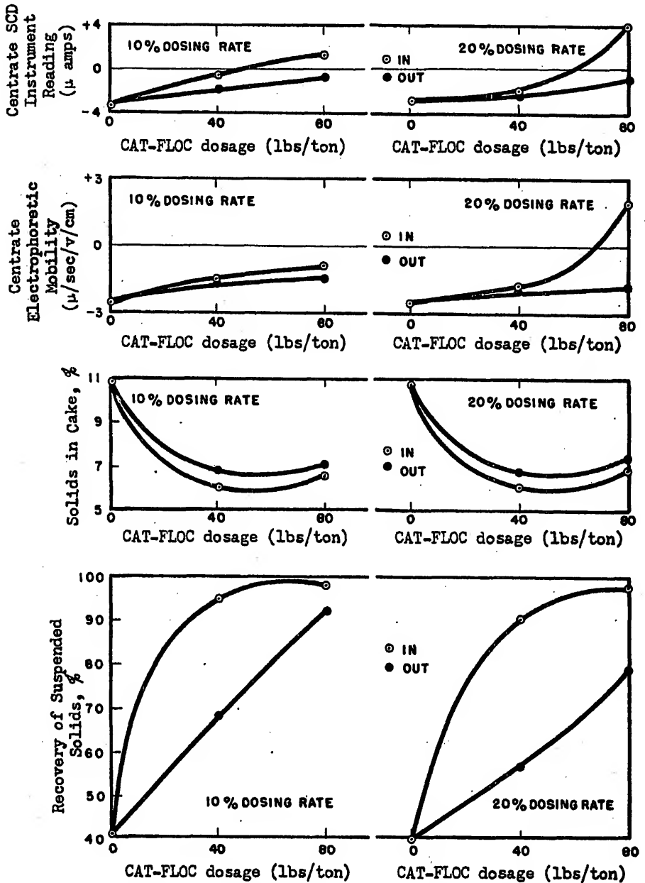
Fig. 32 - Effect of Polymer Dosage, Polymer Dosing Rate, and Location of Polymer Addition on Performance of 6x12 Inch Centrifuge De-watering Waste Sludge, St. Petersburg, Fla.
