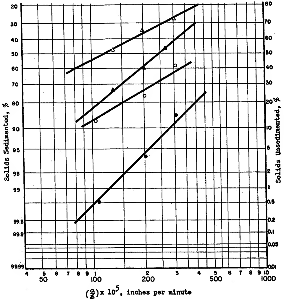
Fig. 39 - Sedimentation Performance Versus Parameter \frac{g}{\text{min}} for Bird Solid Bowl Centrifuges Dewatering Return Activated Sludge, Treasure Island, Fla.
