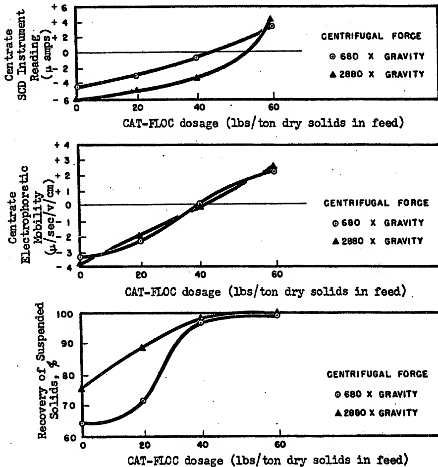
Fig. 19 - Effect of Centrifugal Force and Polymer Dosage on Electrophoretic Mobility and Streaming Current Response of Particles in Centrate When Dewatering Digested Sludge, University of Florida.
