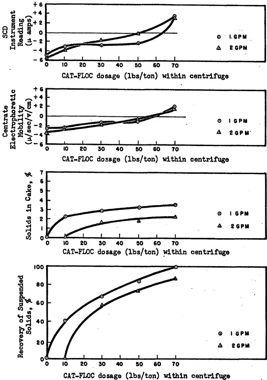
Fig. 27 - Effect of Centrifugal Force, Feed Rate, and Polymer Dosage on Performance of 6x12 Inch Centrifuge Dewatering Return Activated Sludge, University of Florida.
