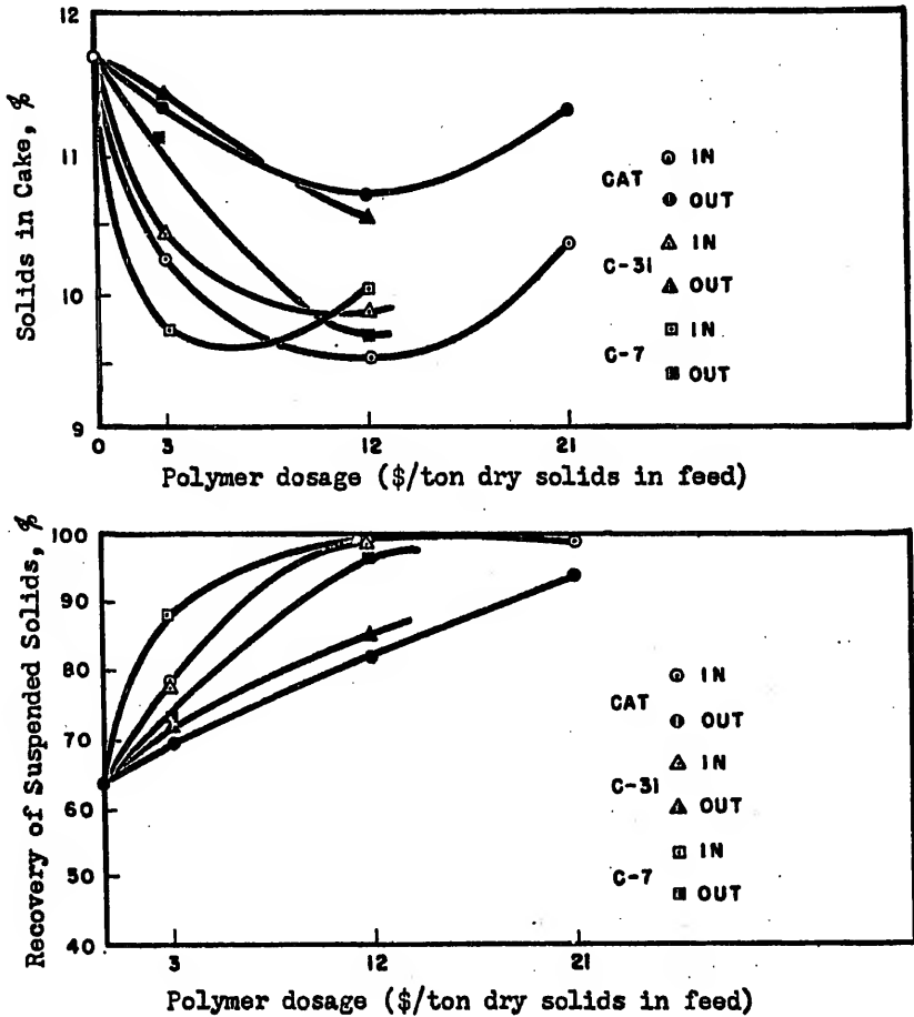
Fig. 18 - Effect of Three Cationic Polymers and Location of Polymer Addition on the Performance of 6x12 Inch Centrifuge Dewatering Digested Sludge, University of Florida.
