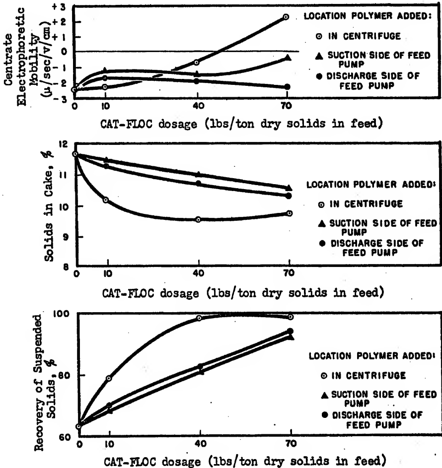
Fig. 16 - Effect of Polymer Dosage and Location Polymer Added on Performance of 6x12 Inch Centrifuge Dewatering Digested Sludge, University of Florida.
