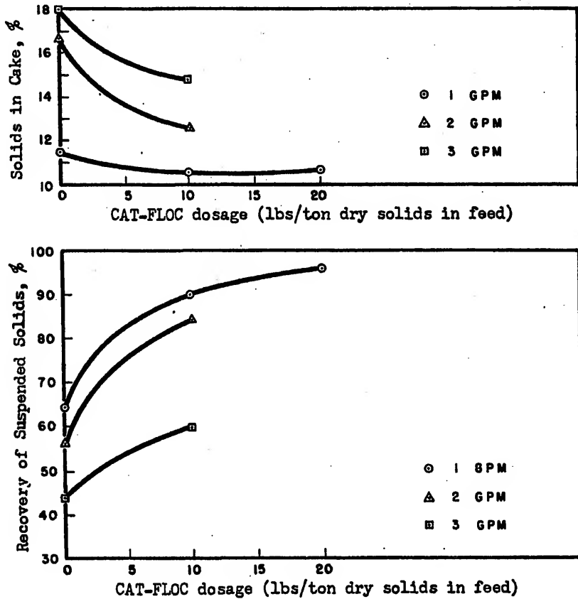
Fig. 36 - Effect of Sludge Feed Rate and Polymer Dosage on Performance of 6x12 Inch Centrifuge Dewatering Raw Sludge, University of Florida.
