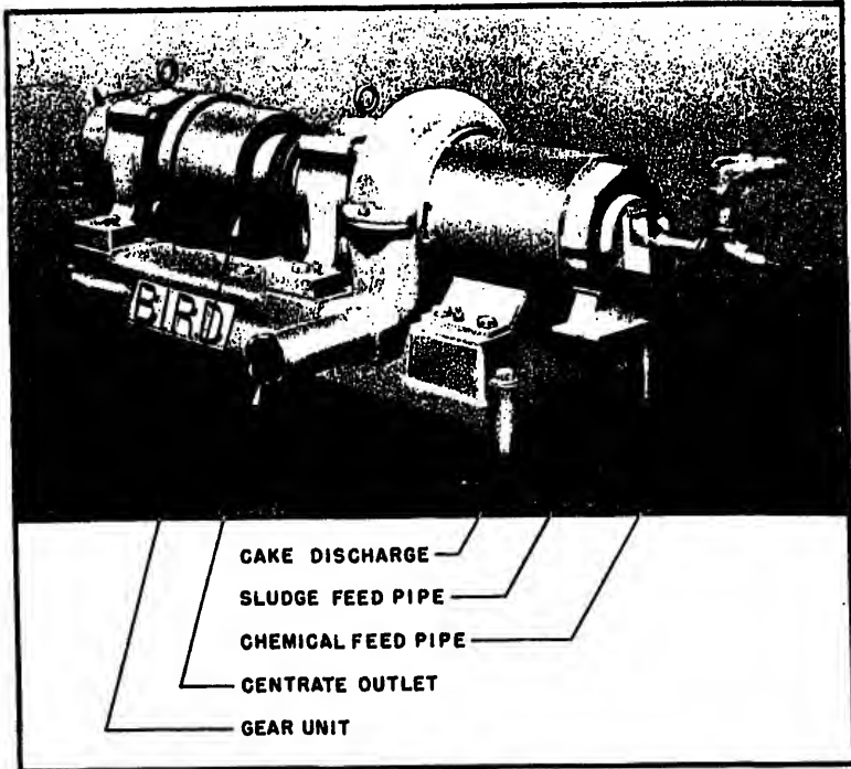
Fig. 11 - Bird 6x12 Inch Solid Bowl Continuous Centrifuge.
