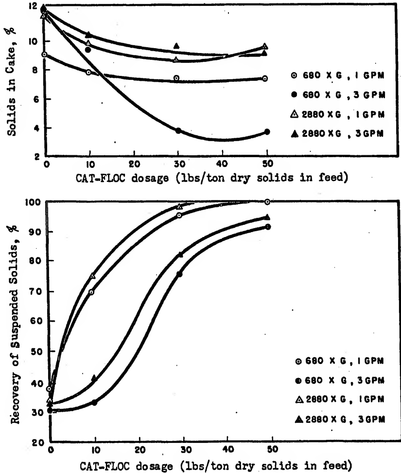
Fig. 31 - Effect of Centrifugal Force, Sludge Feed Rate, and Polymer Dosage on Performance of 6x12 Inch Centrifuge Dewatering Waste Sludge, St. Petersburg, Fla.
