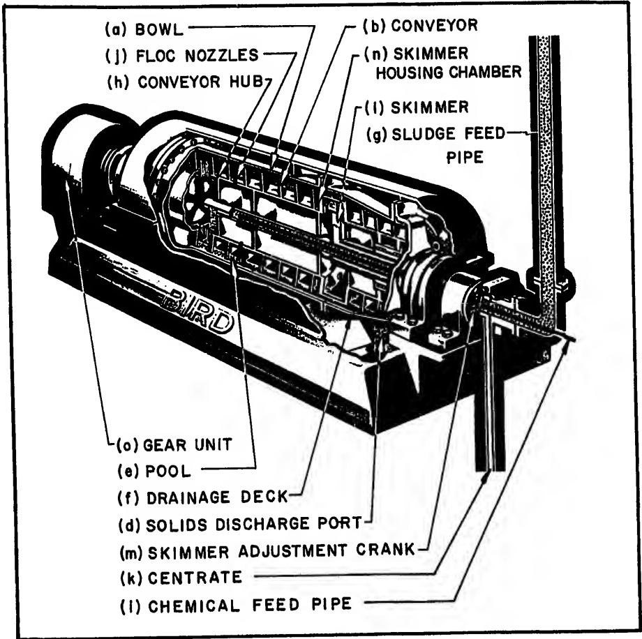
Fig. 9 - Bird Solid Bowl Continuous Centrifuge With Concurrent Flow.
