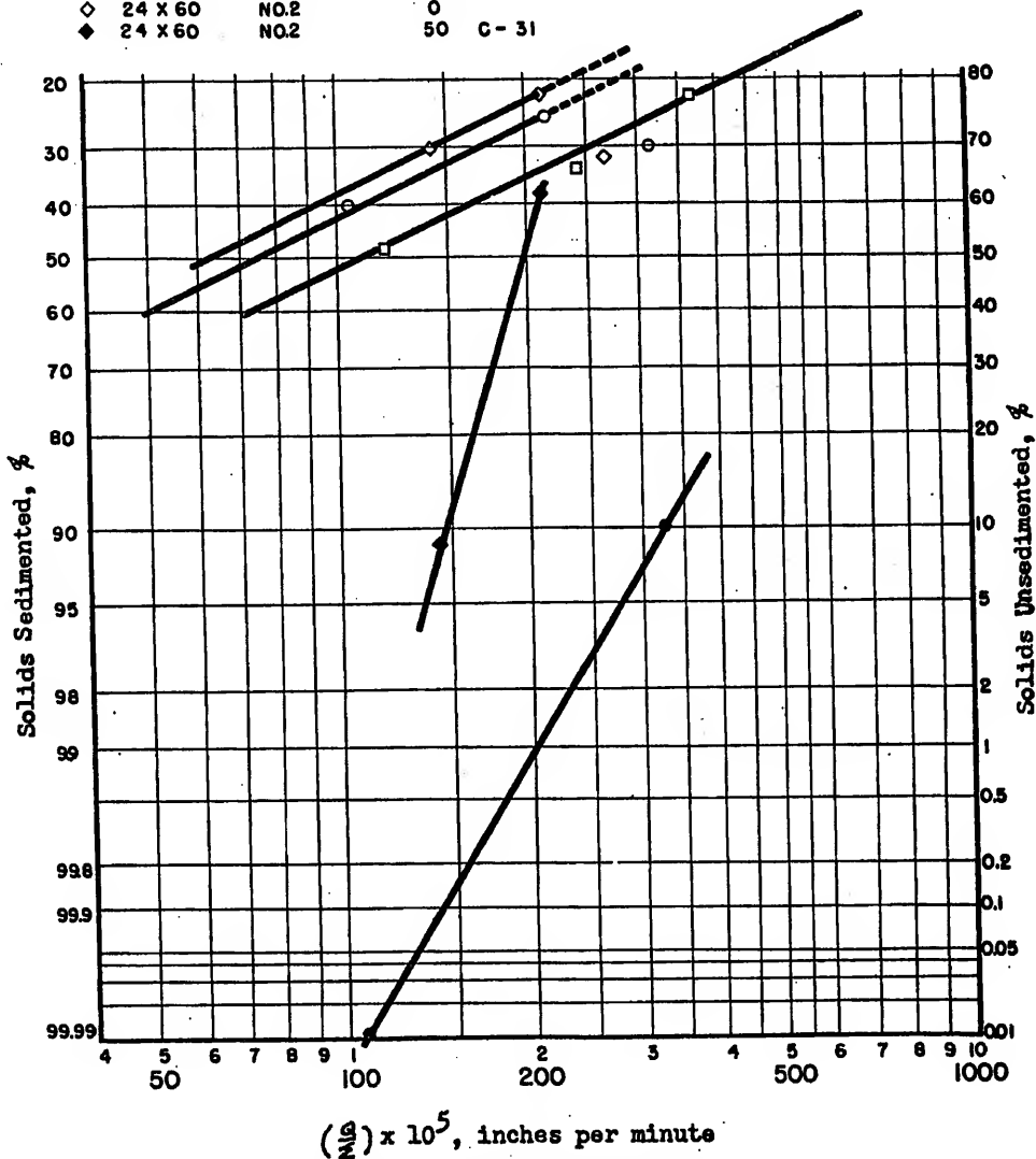
Fig. 40 - Sedimentation Performance Versus Parameter \frac{G}{M} for Bird Centrifuge Dewatering Waste Sludge, St. Petersburg, Fla.
