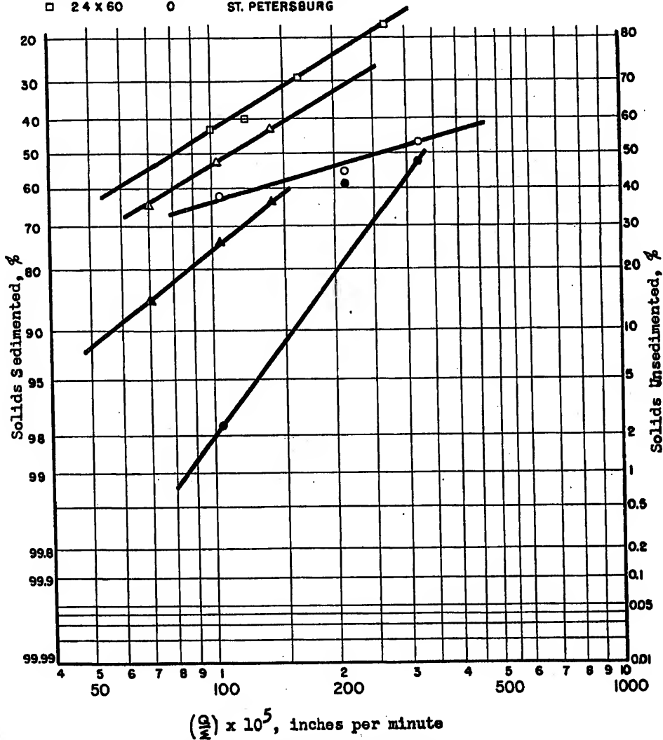
Fig. 38 - Sedimentation Performance Versus Parameter \frac{RPM}{min} for Bird Solid Bowl Centrifuges Dewatering Digested Sludge.
