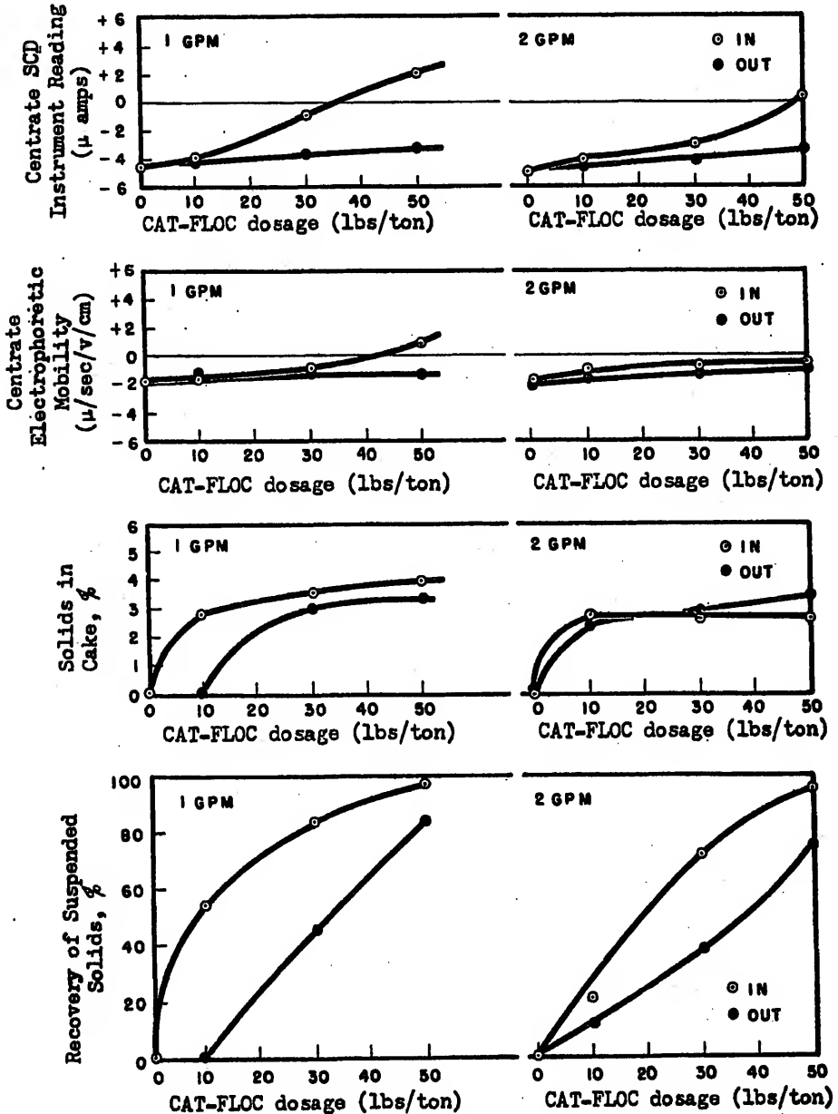
Fig. 25 - Effect of Feed Rate, Polymer Dosage, and Location Polymer Added on Performance of 6x12 Inch Centrifuge Dewatering Return Activated Sludge, University of Florida.
