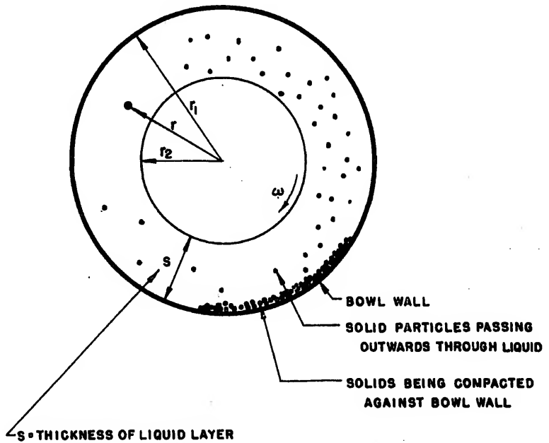
Fig. 3 - Cross Section of a Cylindrical Centrifuge Bowl Showing the Separating Mechanism.
