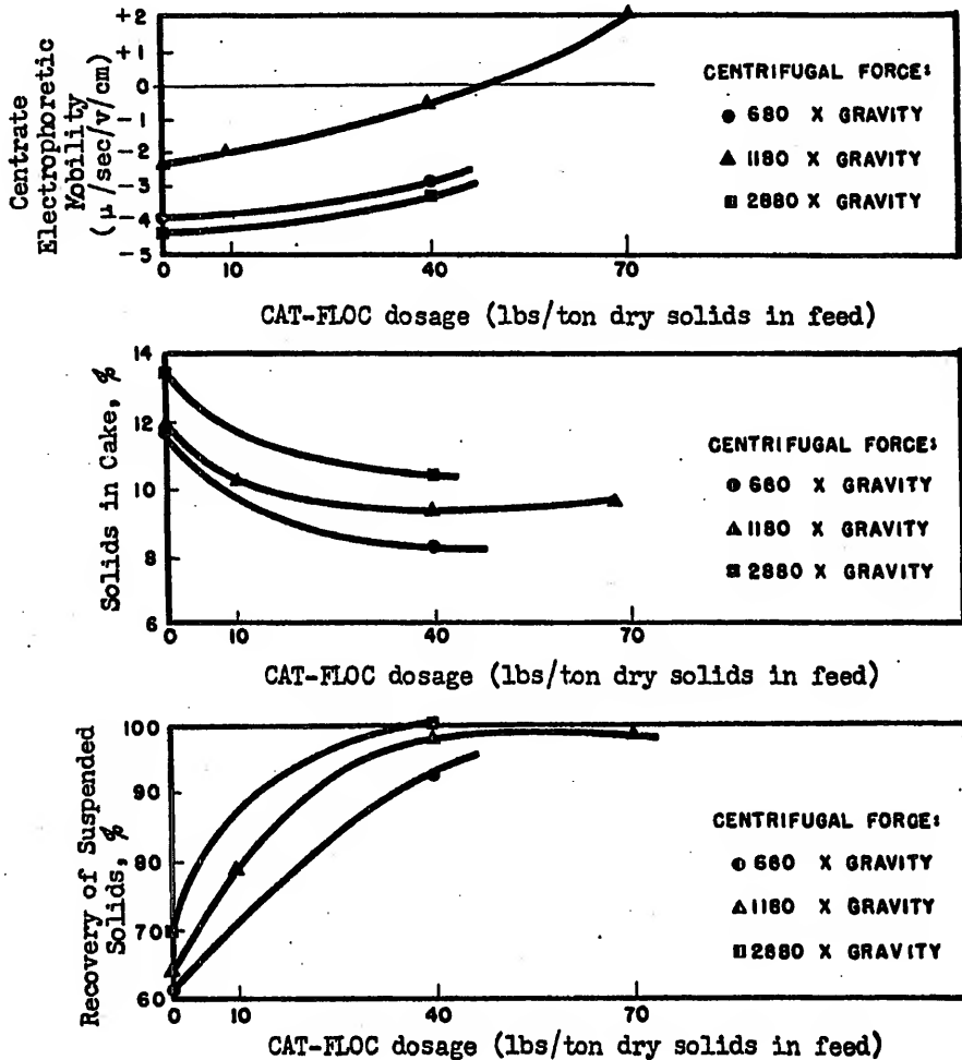
Fig. 17 - Effect of Centrifugal Force and Polymer Dosage on Performance of 6x12 Inch Centrifuge Dewatering Digested Sludge, University of Florida.
