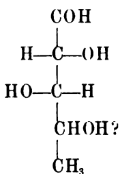
Methyltetrose
