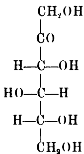
l-Sorbinose
