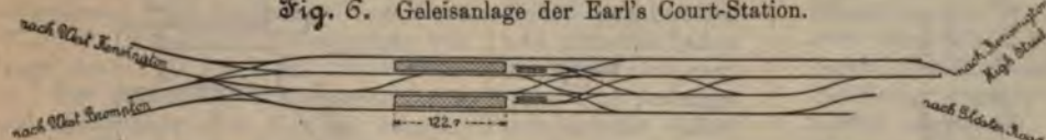
Fig. 6. Geleisanlage der Earl's Court-Station.
