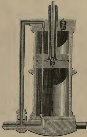
Fig. 139. Barrel of Bianchi's Air-pump.
