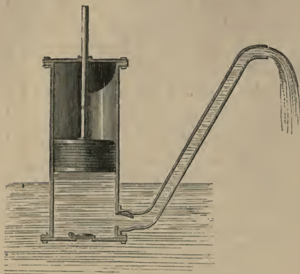
Fig. 161.—Forcing-pump.
