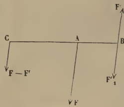
Fig. 8.—Parallel forces in Opposite Directions.
