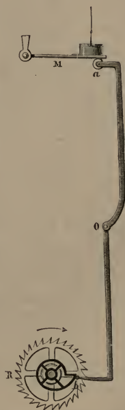
Fig. 30.—Detent in Attwood's Machine.
