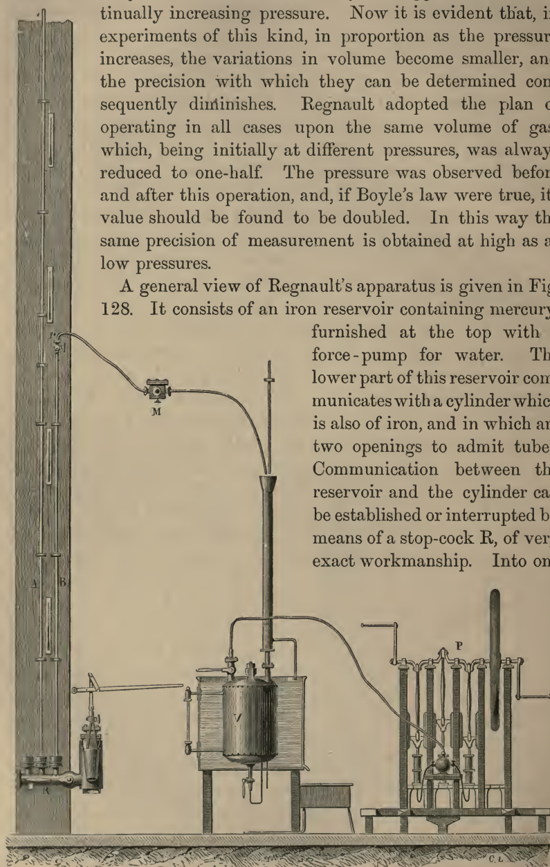
Fig. 128.—Regnault's Apparatus for Testing Boyle's Law.
