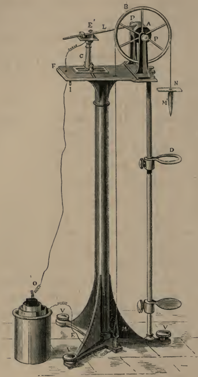
Fig. 31.—Bourbouze's Modification of Atwood's Machine.
