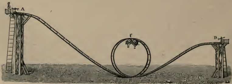
Fig. 38.—Centrifugal Railway.
