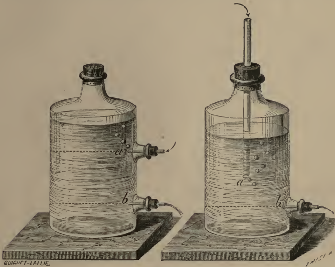
Fig. 181.—Mariotte's Bottle.
