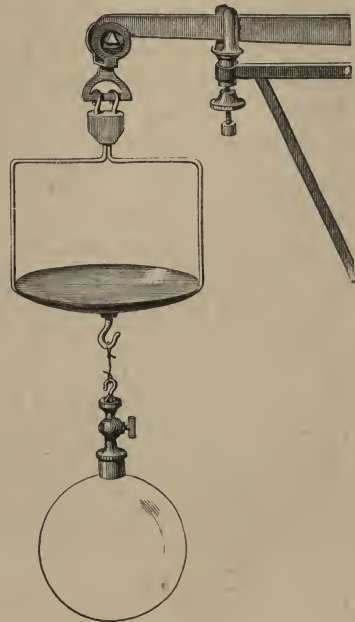
Fig. 106.—Weight of Air.
