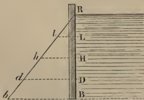
Fig. 63.—Centre of Pressure.
