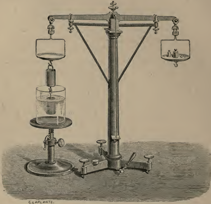
Fig. 66.—Experimental Verification of Principle of Archimedes.
