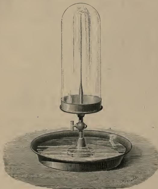
Fig. 143.—Fountain in Vacuo.
