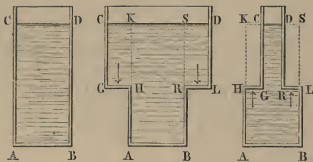
Fig. 60.—Hydrostatic Paradox.
