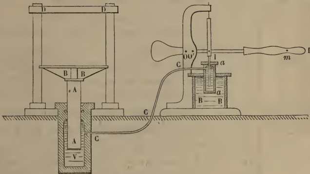
Fig. 167.—Bramah Press.
