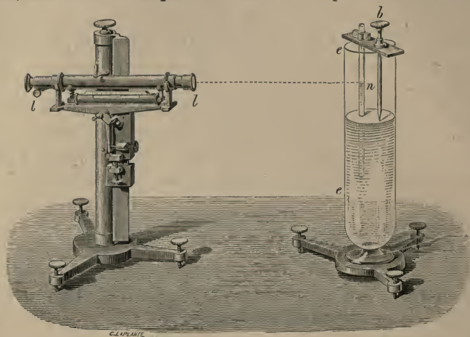
Fig. 104.—Verification of Law of Diameters.
