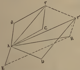
Fig. 4.—Composition of any Number of Forces.
