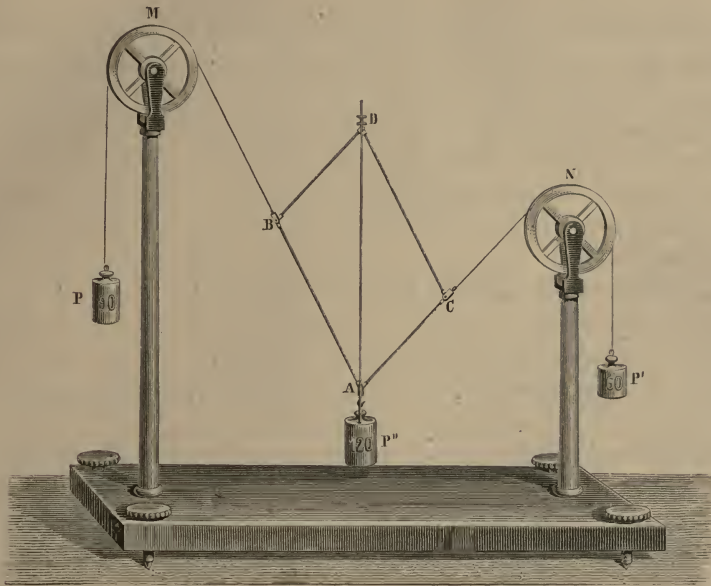
Fig. 3.—Gravesande's Apparatus.
