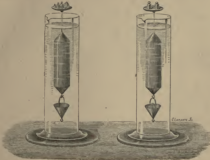
Fig. 78.—Nicholson's Hydrometer.
