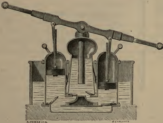
Fig. 162.—Fire engine.
