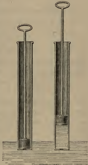
Fig. 157.—Principle of Suction-pump.
