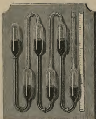
Fig. 121.—Fahrenheit's Barometer.
