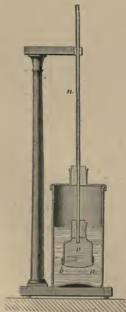
Fig. 105.—Endosmometer.
