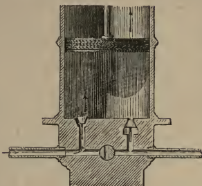
Fig. 150.—Barrel of Condensing Pump.
