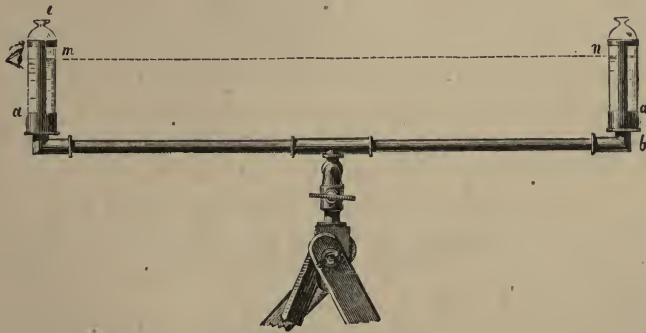
Fig. 90.—Water-level.
