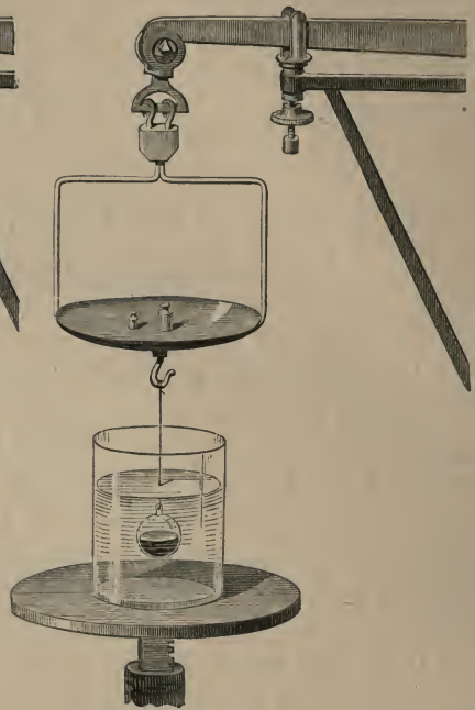
Fig. 77.—Specific Gravity of Liquids.
