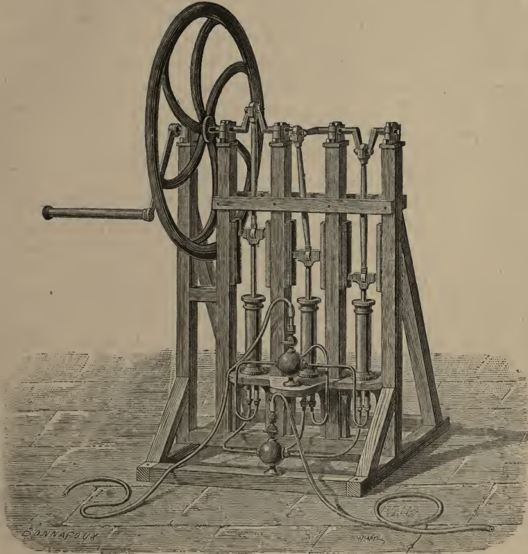
Fig. 152.—Connected Pumps.
