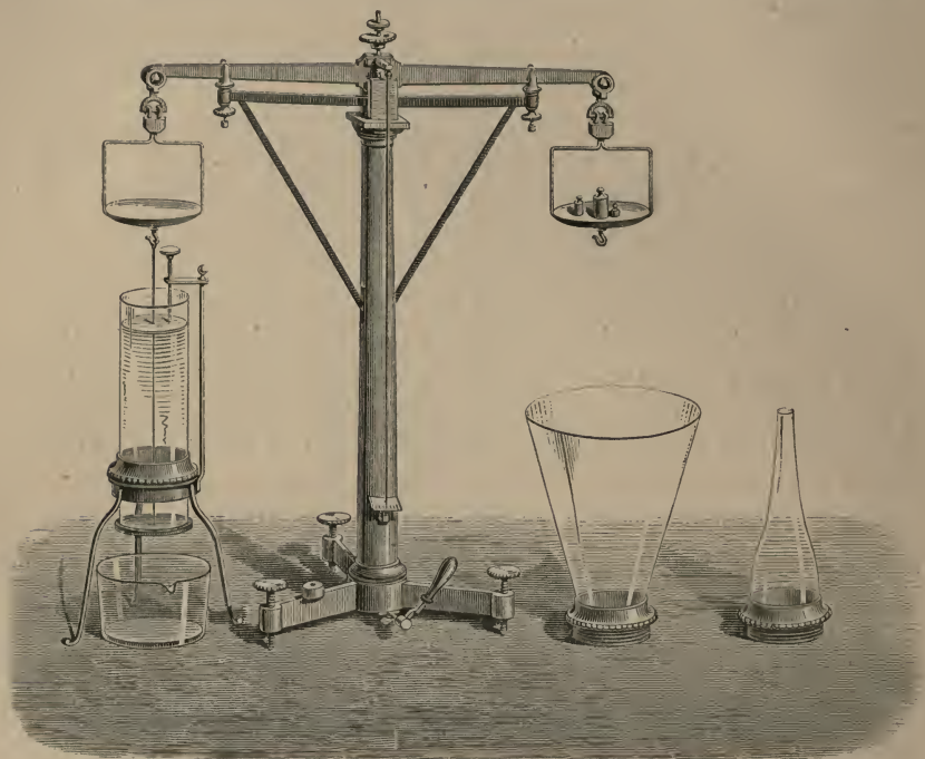
Fig. 57.—Experiment of Pascal's Vases.
