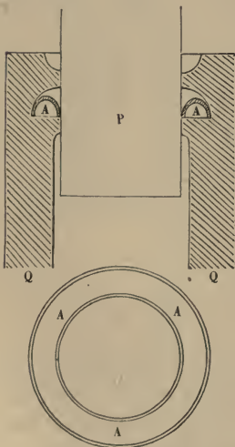
Fig. 168.—Cup—Leather.
