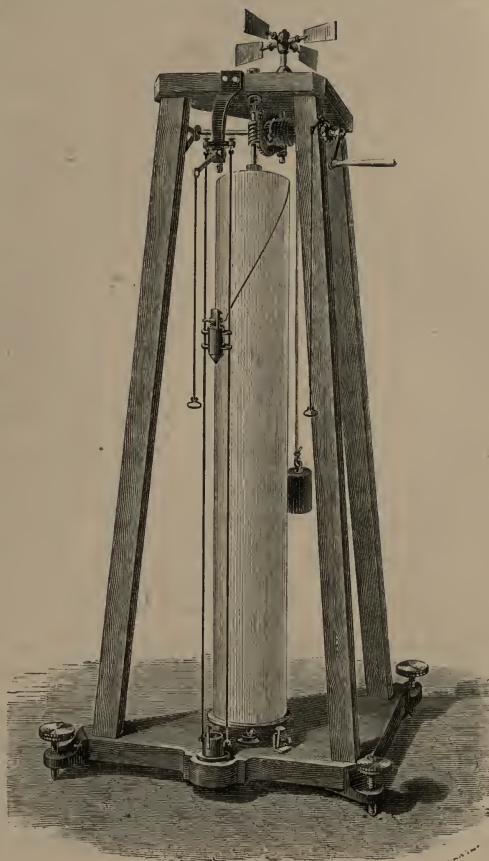
Fig. 32.—Morin's Apparatus.
