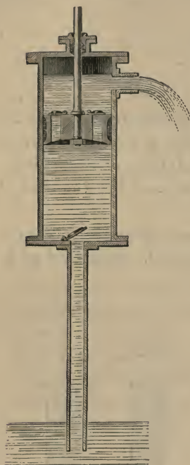
Fig. 158.—Suction-pump.
