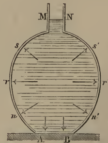
Fig. 59.—Total Pressure.
