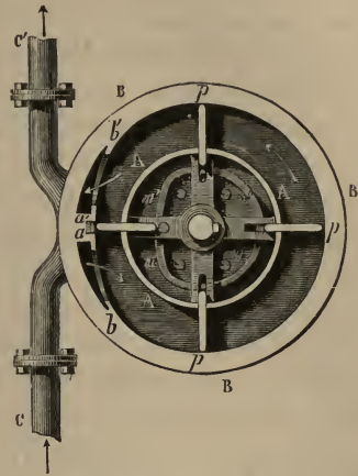
Fig. 166.—Rotatory Pump.
