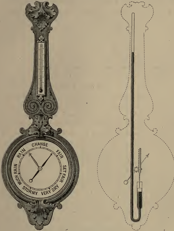
Fig. 118.—Wheel Barometer
