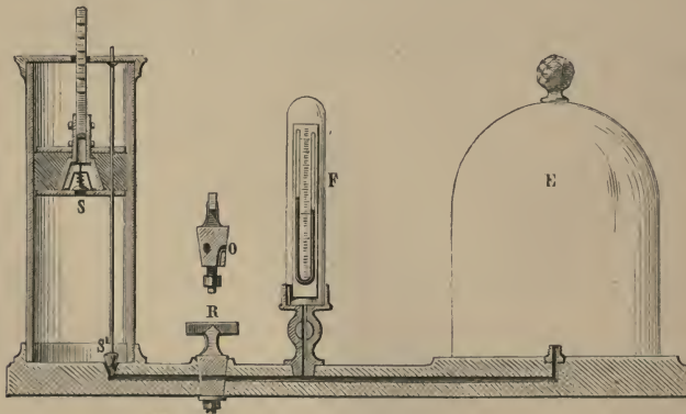
Fig. 135.—Air-pump.
