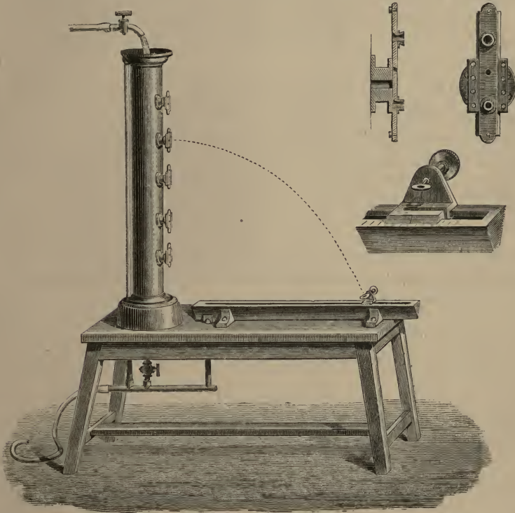
Fig. 169.—Apparatus for verifying Torricelli's Theorem.
