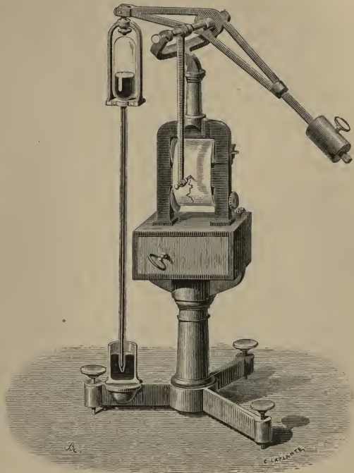
Fig. 120.—Counterpoised Barometer.
