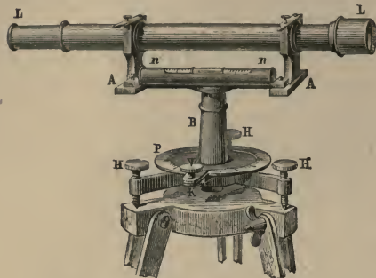
Fig. 96.—Spirit-level with Telescope.
