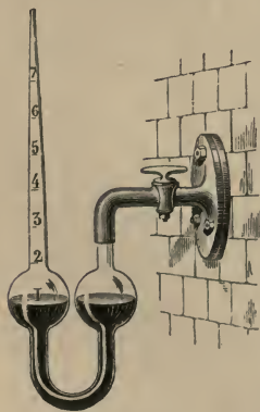
Fig. 132. Compressed-air Manometer.
