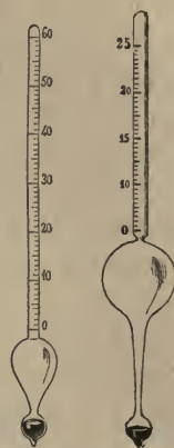
Fig. 82. Beaumé's Hydrometer. Fig. 83. Alcoholimeter.
