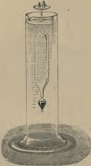
Fig. 79.—Fahrenheit's Hydrometer.
