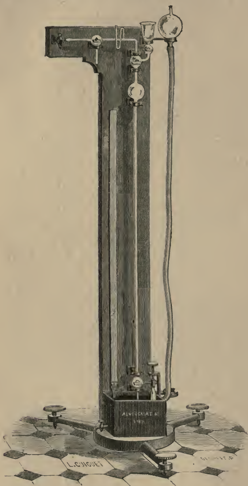
Fig. 146.—Geissler's Machine.
