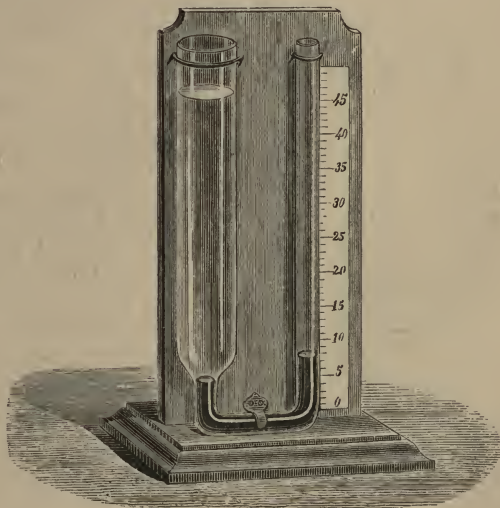
Fig. 98.—Equilibrium of Two Fluids in Communicating Vessels.
