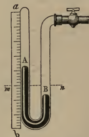
Fig. 131.—Compressed-air Manometer.
