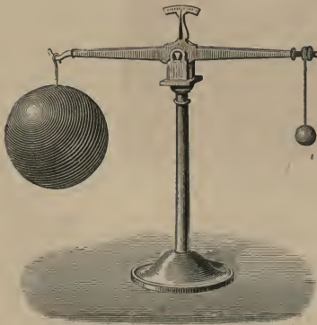
Fig. 153.—Baroscope.
