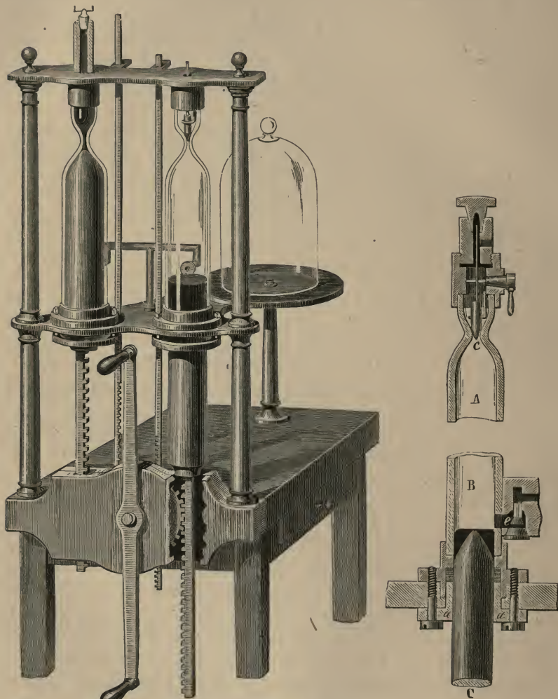
Fig. 145.—Kravogl's Air-pump.
