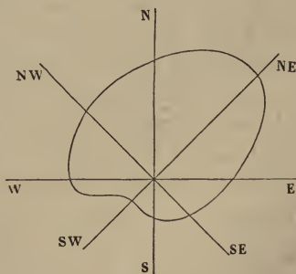
Fig. 124. Barometric Rose of Winds at Paris.
