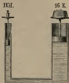
Fig. 50.—Principle of the Hydraulic Press.
