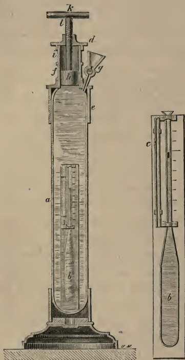
Fig. 12.—Ersted's Piezometer.
