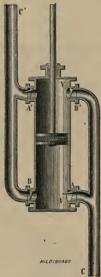
Fig. 165. Double-action Pump.
