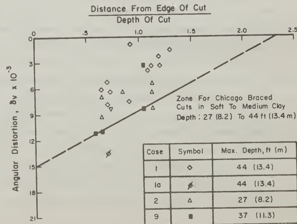
Fig. 2.16 Angular Distortion for Braced Cuts in Chicago
