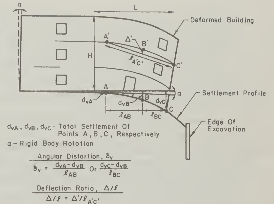
Fig. 3.1 Building Deformation Caused by Settlement in Response to Opencutting
