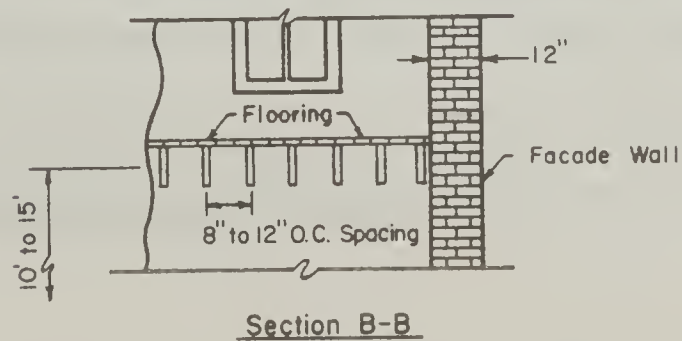
Fig. 4.1 Typical Brick-Bearing Wall Structure
