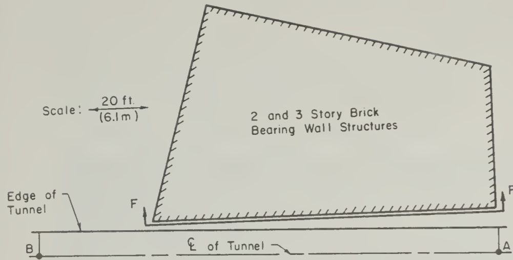
a) Plan View of Tunnel and Buildings Along Path of Tunnel
