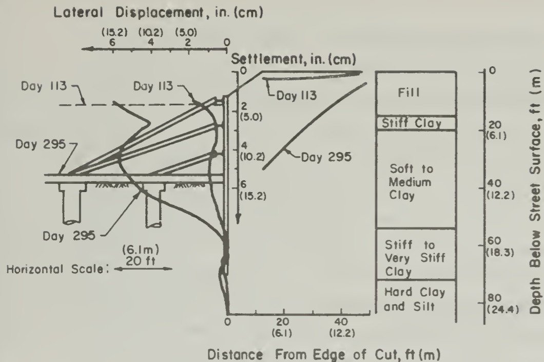
Fig. 2.13 Soil Displacements for Case 9
