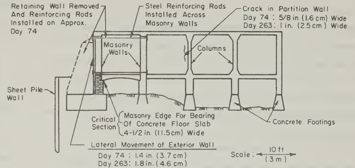
a) Detail of Rail Station
