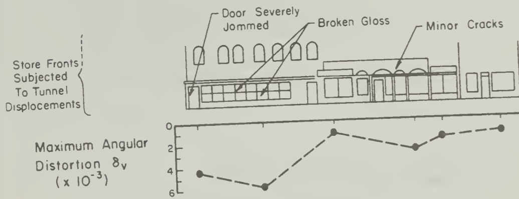
b) Profile of Store Fronts (Section F-F) With Maximum Angular Distortion and Location of Damage
