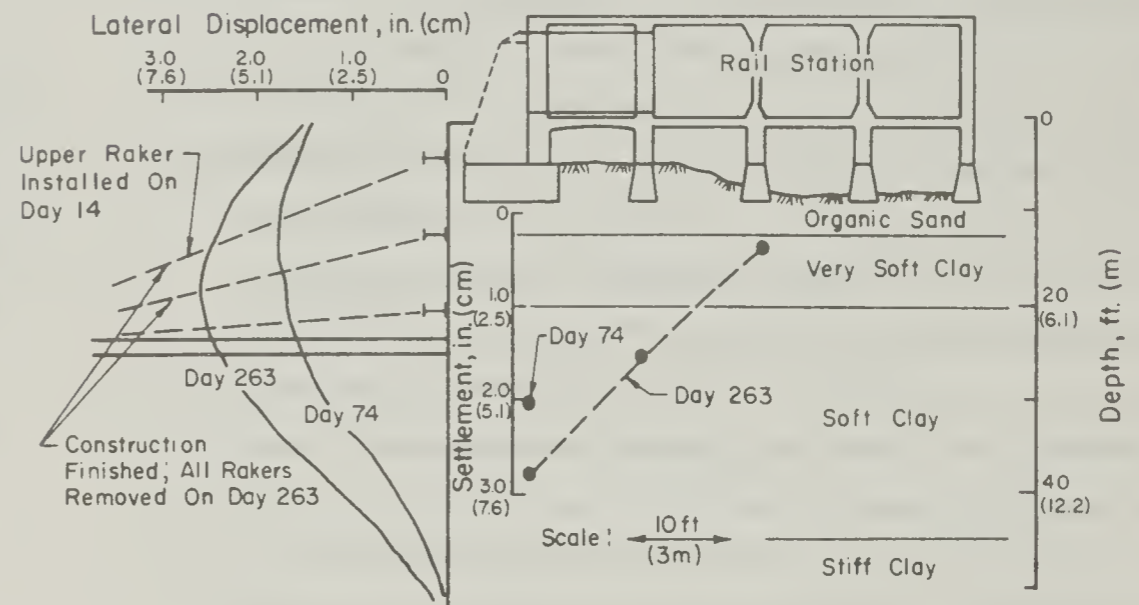
b) Vertical and Lateral Displacement Profile
