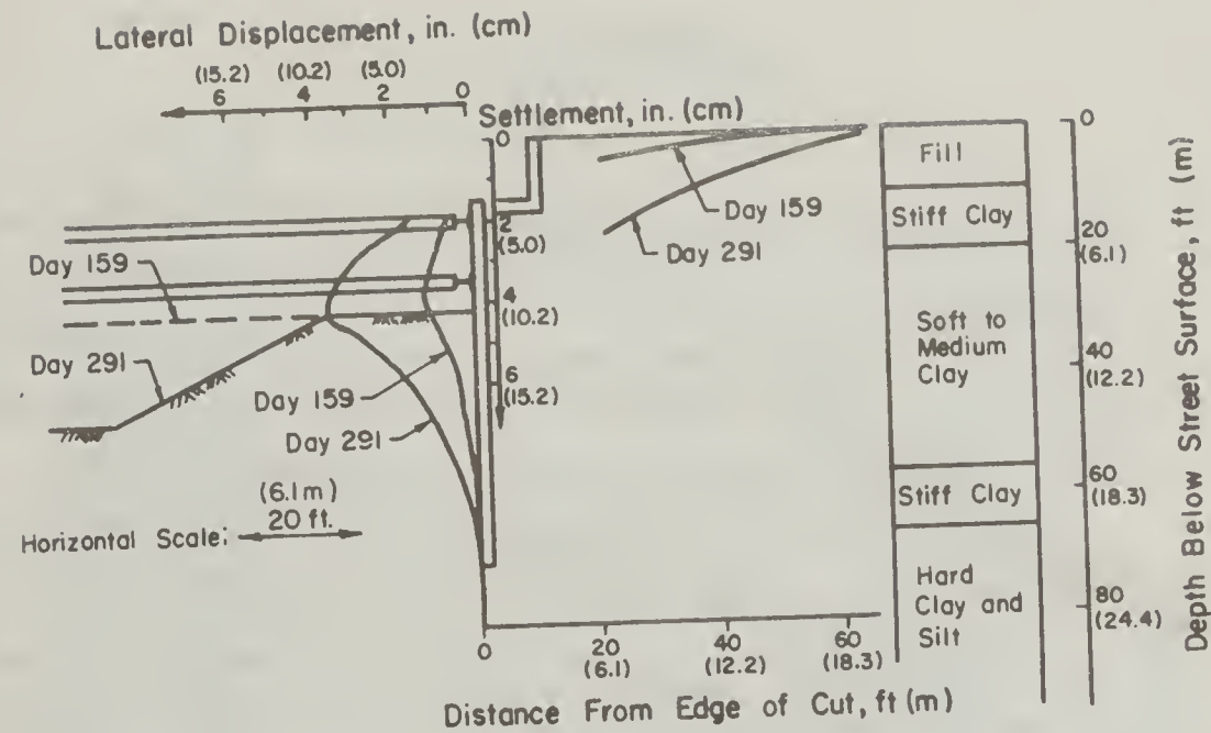
Fig. 2.11 Soil Displacements for Case 1
