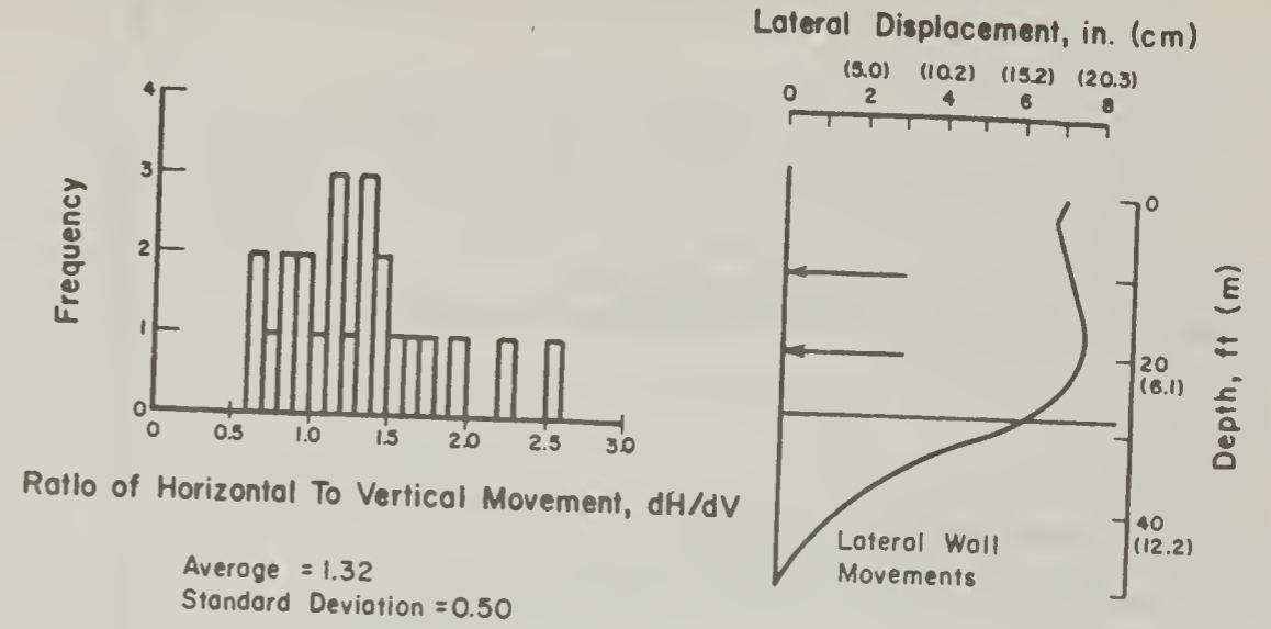
Fig. 2.21 Ratios of Horizontal to Vertical Ground Movement for Case 4
