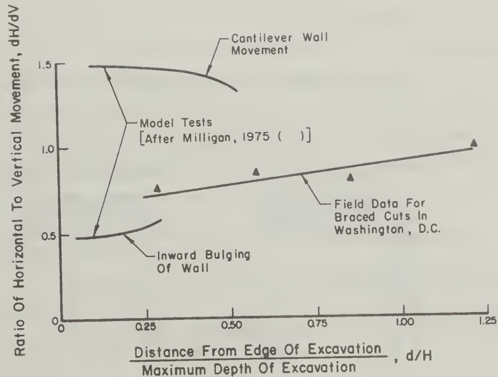
Fig. 2.8 Ratio of Horizontal to Vertical Ground Movements for Model Tests and Excavations in Washington, D. C.
