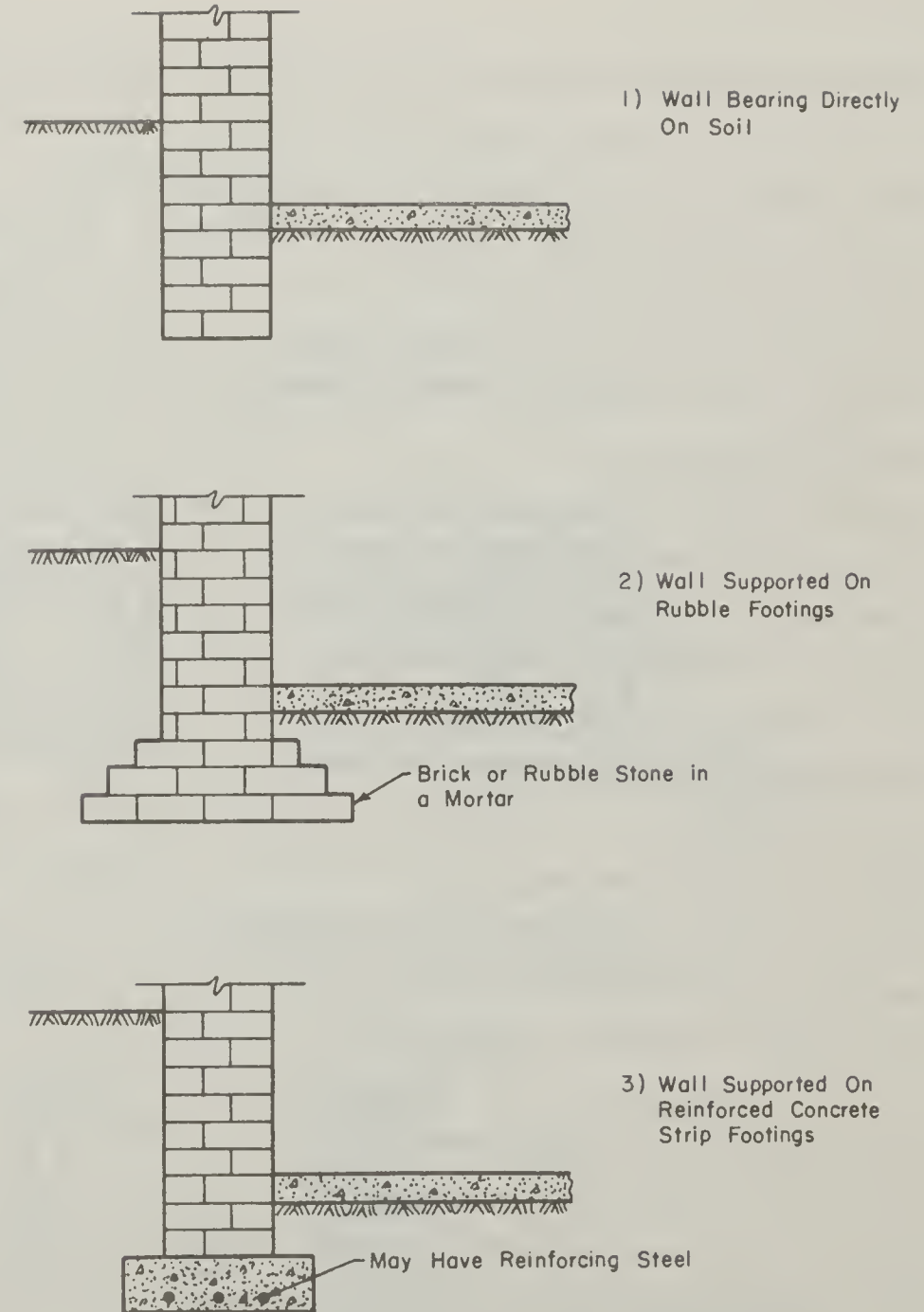
Fig. 4.3 Typical Foundations for Brick-Bearing Wall Structures
