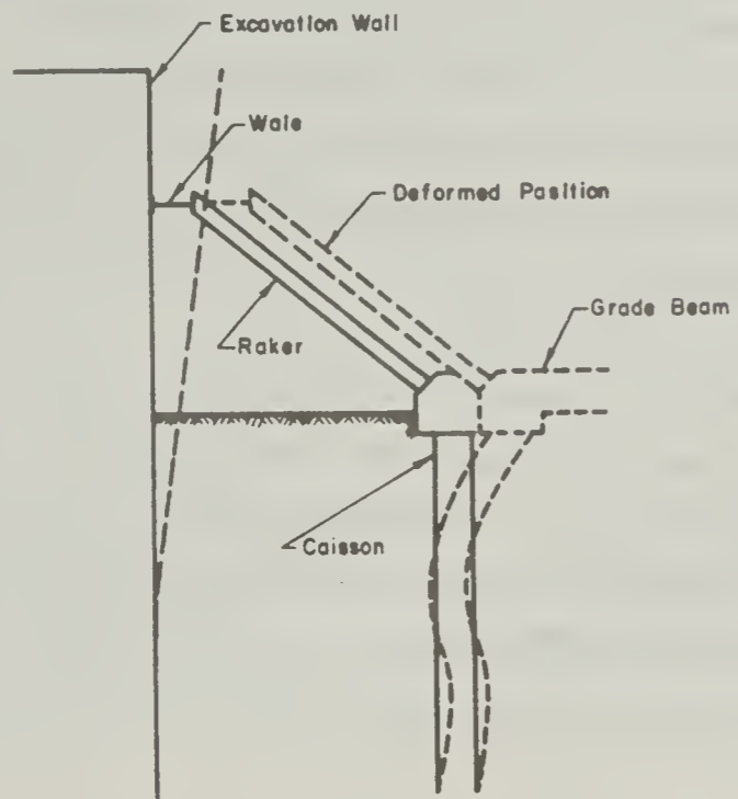
Fig. 2.13 Soil Displacements for Case 9
