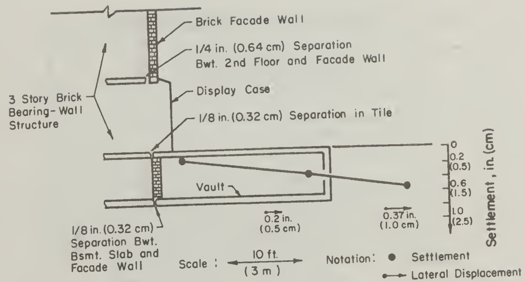
a) Detail of 3-story Building
