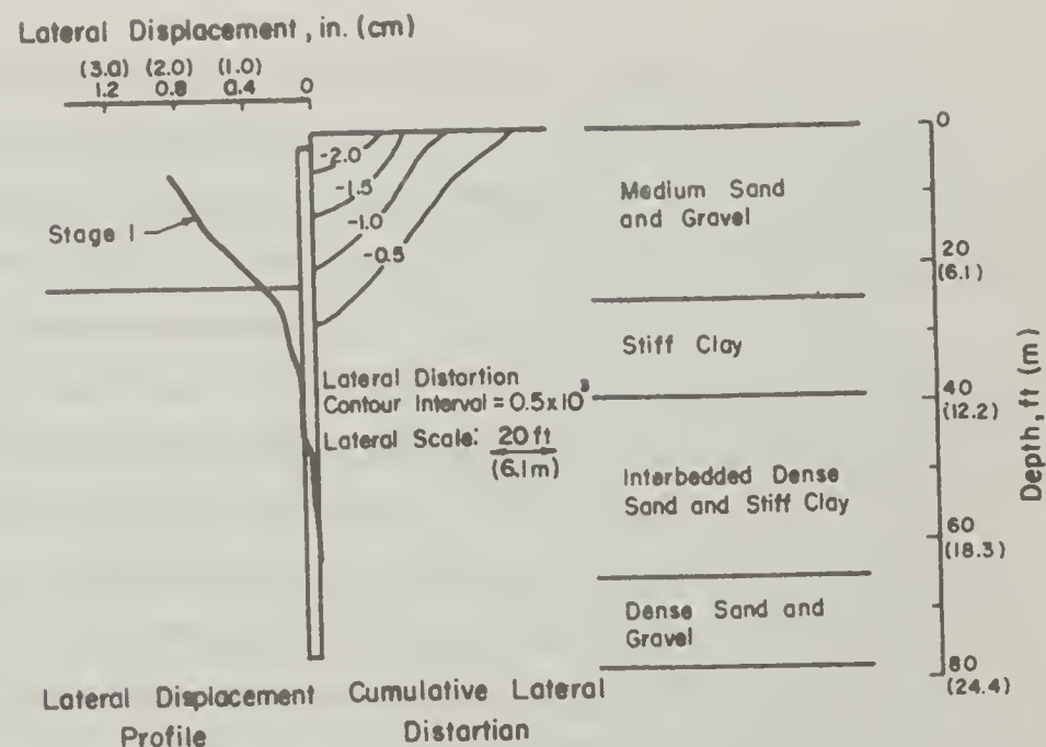
Fig. 2.4 Lateral Distortion Corresponding to Stage 1: Excavation Before Installation of Braces
