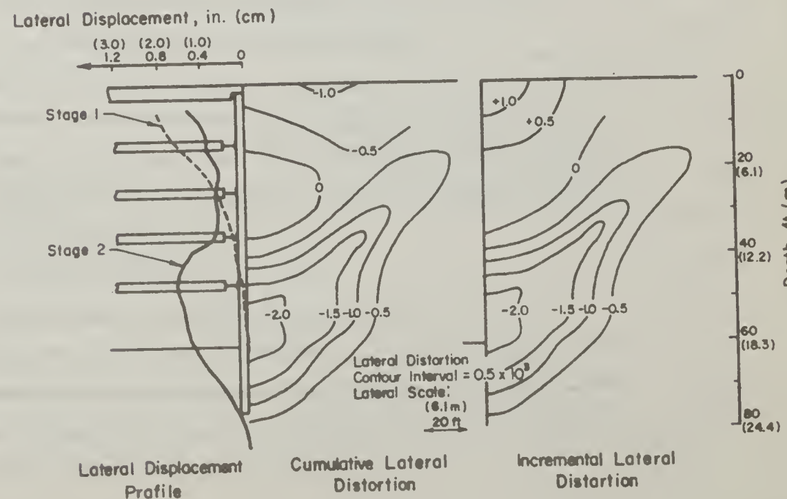
Fig. 2.5 Lateral Distortion Corresponding to Stage 2: Excavation to Subgrade
