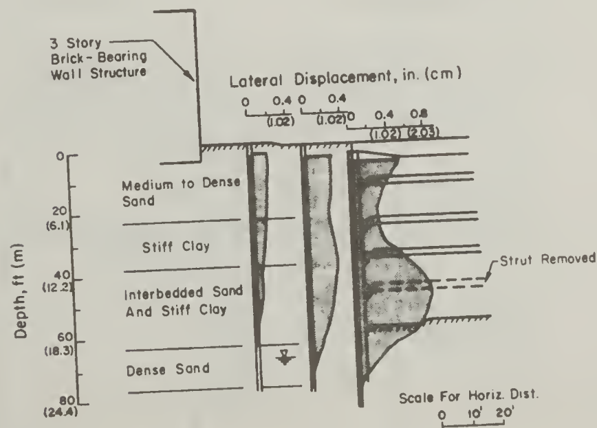
b) Lateral Displacement Profiles
