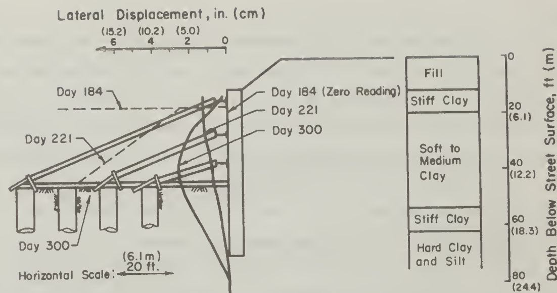
Fig. 2.15 Soil Displacements for Case 7
