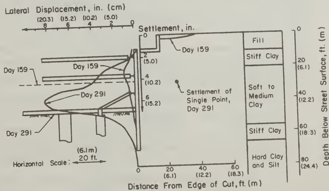
Fig. 2.12 Soil Displacements for Case 1a
