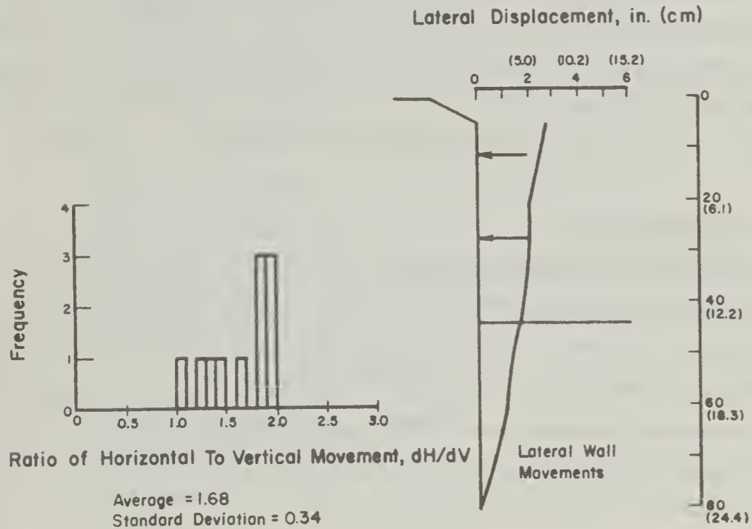
Fig. 2.20 Ratios of Horizontal to Vertical Ground Movement for Case 3
