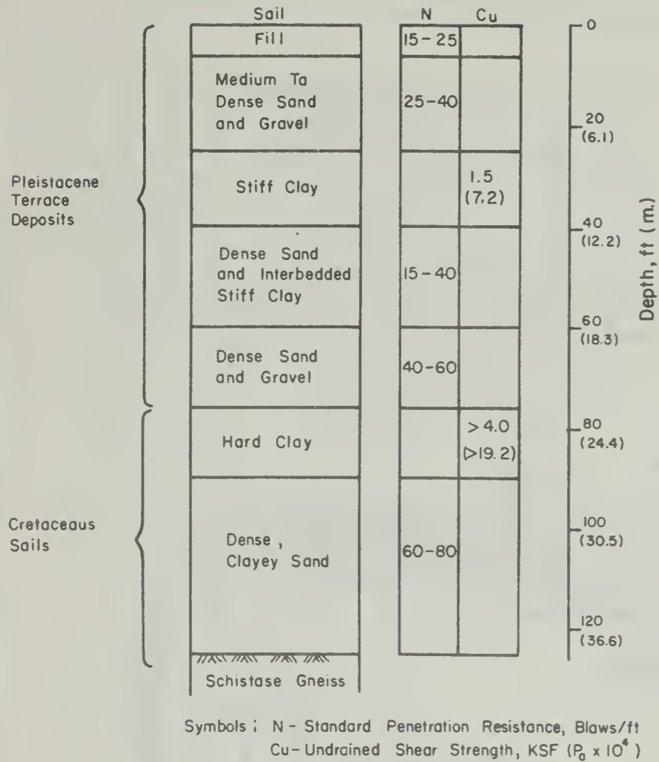
Fig. 2.1 Soil Profile for Braced Excavations in Washington, D. C.
