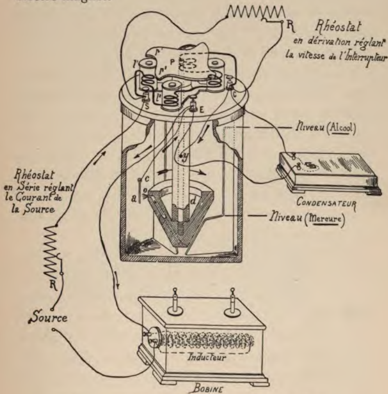
FIG. 13.—DIAGRAM OF AUTONOME INTERRUPTER.
