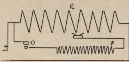
FIG. 18A.—SHUNT RESISTANCE.
