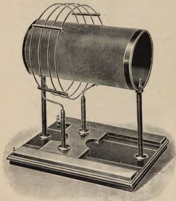
FIG. 29.—D'ARSONVAL RESONATOR.
