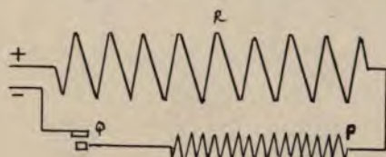
FIG. 18.—SERIES RESISTANCE.
