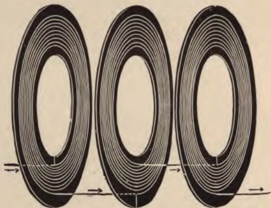
FIG. 8.—DIAGRAM OF JOINTLESS SECTION-WINDING.
