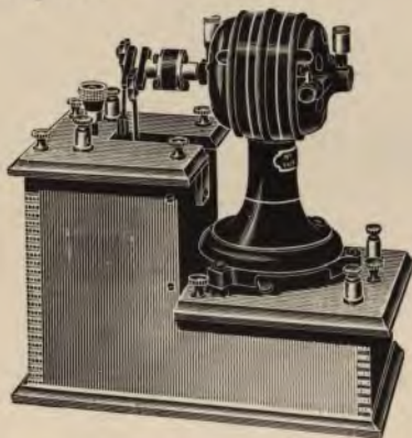
FIG. 16.—DOUBLE-DIPPER INTERRUPTER.
