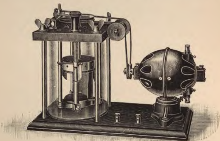
FIG. 11.—TURBINIA JET INTERRUPTER.
