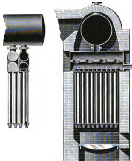
WIEGAND . . . . . 156 H.-P.
