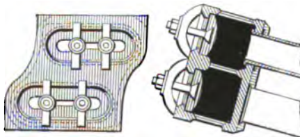
ZELL HEADERS.
