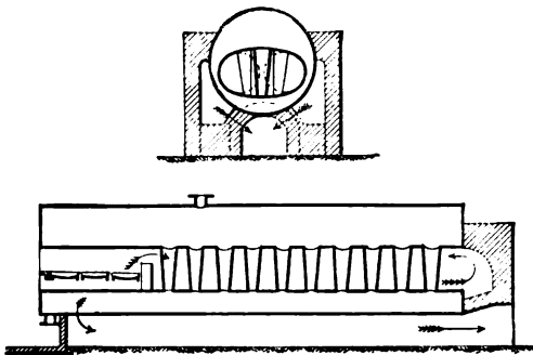
GALLOWAY . . . . . 127 H.-P.
