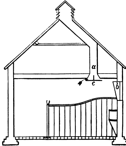
VENTILATING SHAFT.
