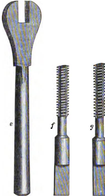
FIG. 9.—SPANNER AND TAPS FOR ROUGHING. e. Spanner. f. g. Taps for tapping. \frac{1}{4} inch size.
