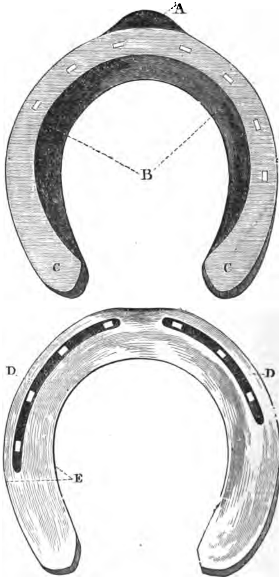
FIG. 2.—CONCAVE-SEATED ENGLISH SHOE FOR OFF FORE FOOT, SHOWING BOTH SURFACES.
