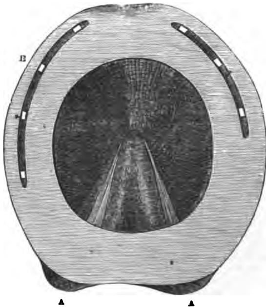
FIG. 5.—BAR SHOE FOR OFF FORE FOOT: FITTED, BUT NOT NAILED ON.
