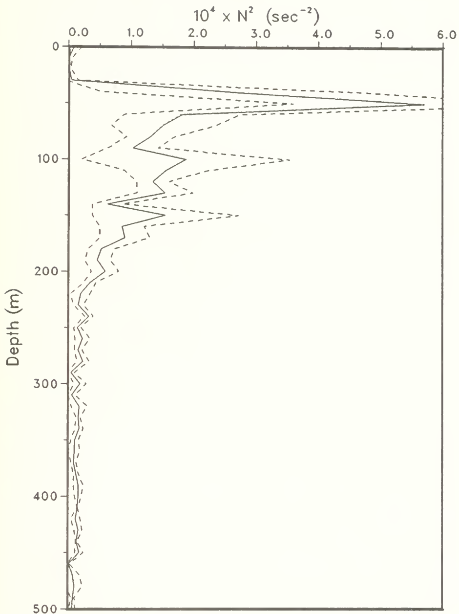
Figure 33: Mean N^2 profile (—), with \pm the standard deviation (----). The N^2 profile from T(z) and S(z) is also shown (.....) (OPTOMA14).
