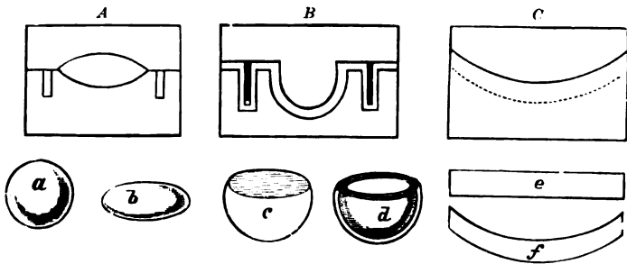
FIG. 4.—A, B, C, molds; a, c, e, original forms of the ice; b, d, f, the forms into which they were molded.
