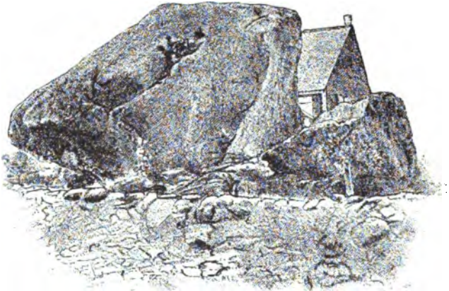
FIG. 60.—Vessel Rock, a glacial boulder in Gilesum, N. H. (C. H. Hitchcock.)
