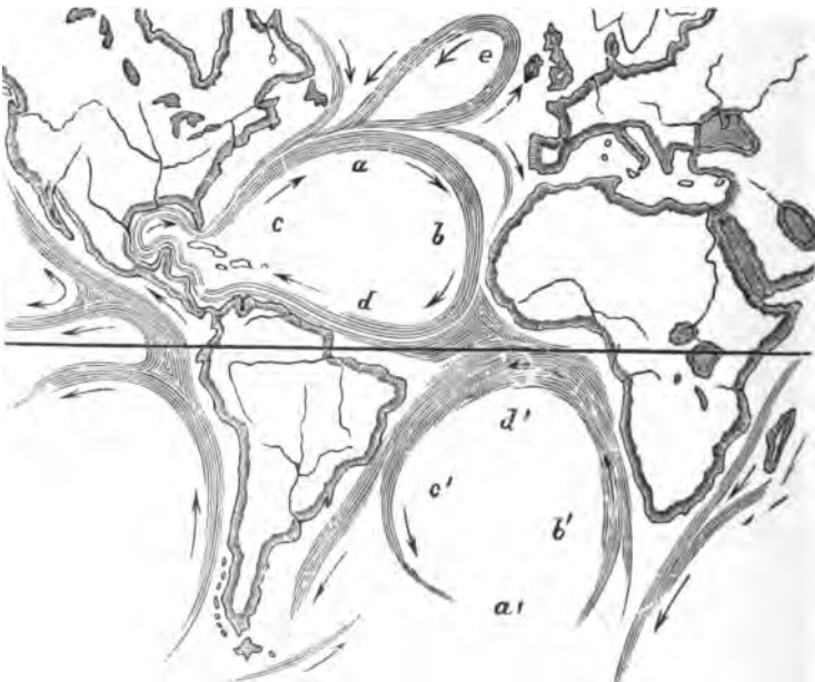
FIG. 104.—Map showing course of currents in the Atlantic Ocean. d and d' are currents set in motion by opposite trade winds; meeting they produce the equatorial current which divides into c and c' continuing on as a and a' and e .
