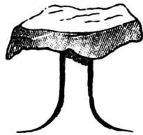
FIG. 9.—Mode of formation of ice-pillars.
