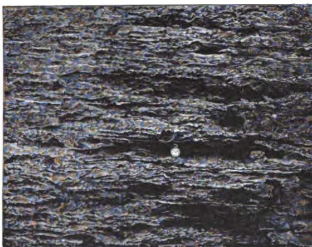
FIG. 99.—Stratification of the loess in a railway cut at Plattsmouth, Nebraska, at a depth of eighty-four feet from the surface. (From photograph furnished by Dr. A. L. Child, of Kansas City, Mo.) (Chamberlin.) (United States Geological Survey.)
