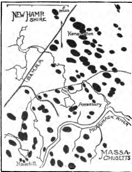
FIG. 75.—Drumlins in northeastern Massachusetts. (Davis.)
