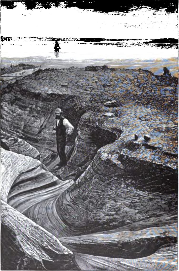
FIG. 66.—Tortuous grooves on Kelly's Island, Lake Erie. United States Geological Survey (Chamberlin).
