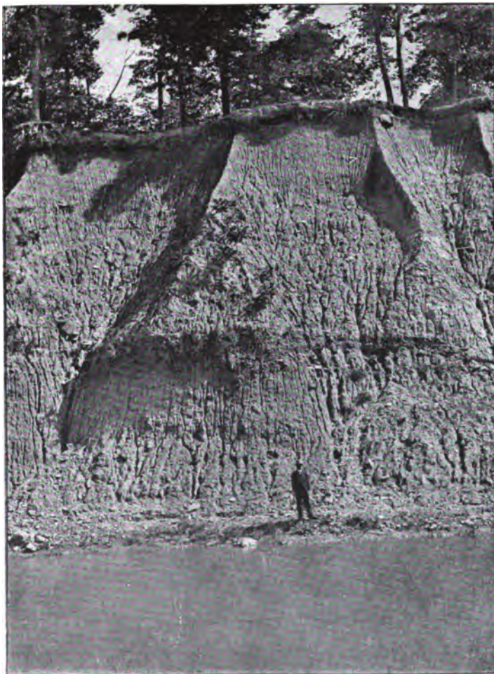
FIG. 118.—Section in till near Darrrtown, Butler County, Ohio, sixty-five feet high. Coarse line of stratification near the middle. Fresh cedar logs at the bottom. (See text.) (United States Geological Survey.) (Wright.)
