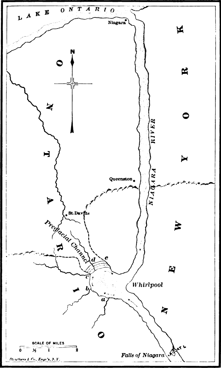
FIG. 109.—Map of the Niagara River below the falls, showing the buried channel from the whirlpool to St. Davids. Small streams a, b, c fall into the main gorge over a rocky escarpment. No rock appears in the channel at d , but the rocky escarpment reappears at e .
