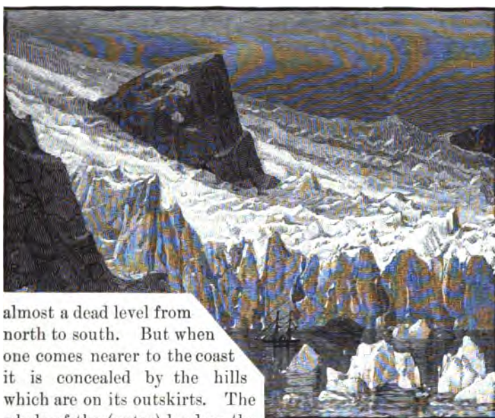
Fig. 31.—A Greenland Glacier, showing the formation of icebergs. From a painting in possession of the New York Geographical Society.
