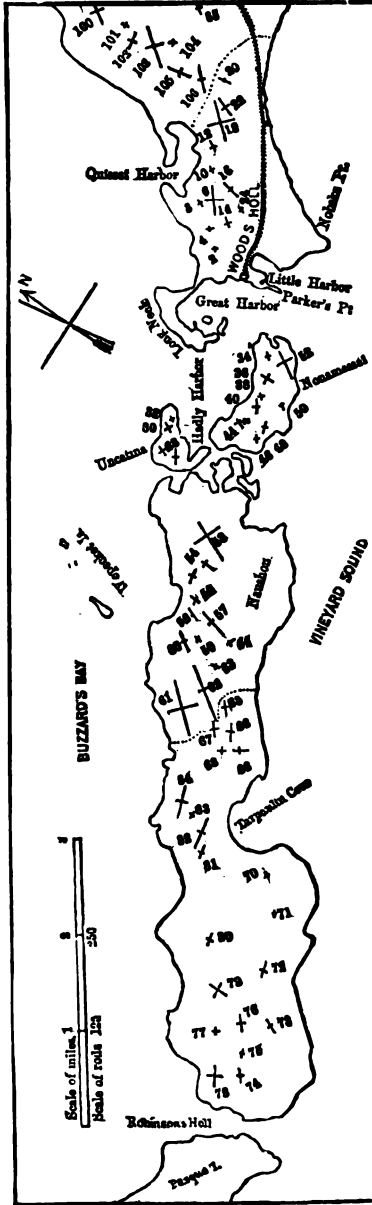
FIG. 53.—Map of kettle-holes on the northern part of the Elizabeth Islands, and in the vicinity of Wood's Hill, Massachusetts, by Professor B. F. Koons. The crosses show the direction of the longer and shorter axes. Nos. 96, 72, 76, 78, 82, 84, 86, 87, 88, 91, 92, 94, 96, 99, 100, 103, 106, 106, are upward of twenty-five rods in diameter; 95 and 108 are upward of fifty rods in diameter; 95 and 108 are about one hundred feet in depth.
