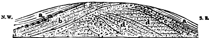
FIG. 89.—Section of kame near Dover, New Hampshire. Length, three hundred feet; height forty feet; base, about forty feet above the Cochecho River, or seventy-five feet above the sea. a, a , gray clay; b , fine sand; c, c , coarse gravel containing pebbles from six inches to one foot and a half in diameter; d, d , fine gravel. (Upham.)
