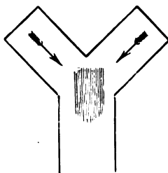
FIG. 8.—Illustrates the formation of veined structure by pressure at the junction of two branches.
