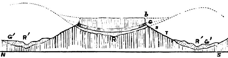
FIG. 143.—Section across Table Mountain, Tuolumne County, California. b , lava; G , gravel; s , slate; R , old river-bed; R' , present river-bed. (Le Conte.)
