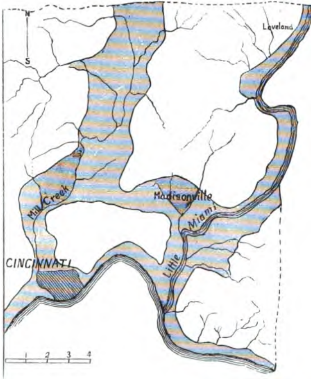
FIG. 130.—Map of the vicinity of Madisonville, Hamilton County, Ohio, where Dr. Metz has found palæolithic implements. (See text.) The unshaded portions represent the high land from three hundred to five hundred feet above the eroded valleys represented by the shaded portions.
