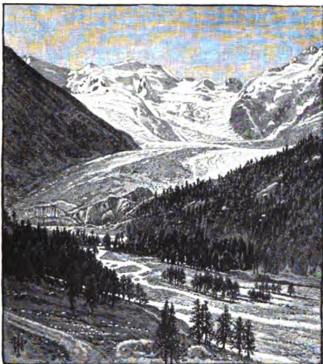
FIG. 82.—Morteratsch Glacier, Grisons Alps. This glacier advances about seven inches per year. Centuries ago chalets stood a mile farther up the valley. In 1868 fragments of these ancient dwellings were washed out from underneath the ice.
