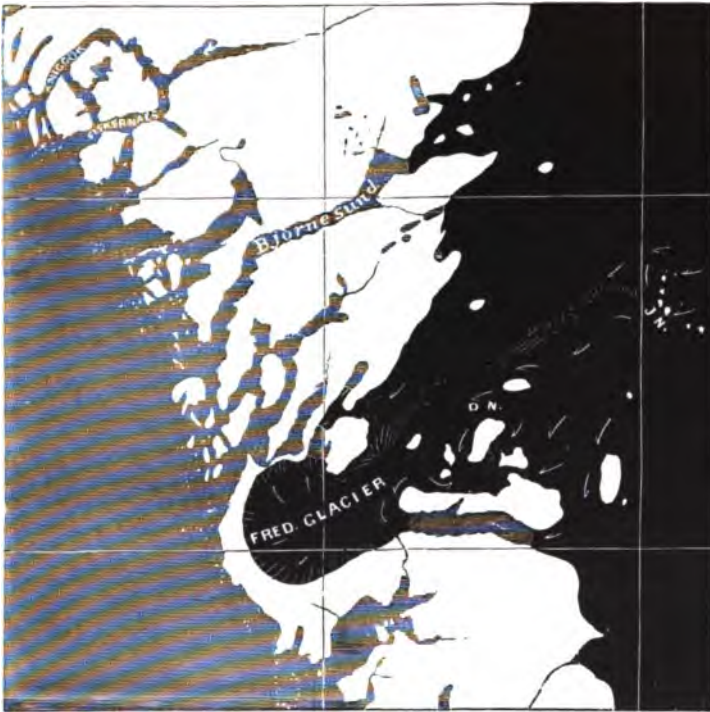
FIG. 30.—Map of Frederikshaab Glacier, between 62° and 63°, showing course of Lieutenant Jensen in 1878 (forty-seven and a half miles). The black part, ice; white, land; shaded, water; J. N., Jensen's nunataks; D. N., Dolager's nunataks; white lines on the black, crevasses; arrows, glacier-flow. Five species of plants were found on the nunataks which still survive on the White Mountains (N. H.). Dana.
