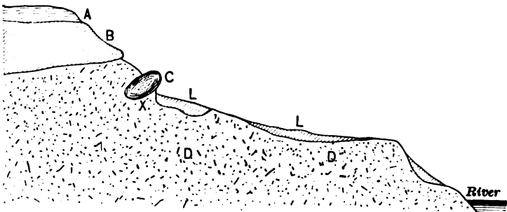
FIG. 133.—Section of glacial gravel at Medora, Indiana, in which Mr. Cresson found the palæolith figured in the text. A, is a deposit of soil three feet in depth; B, modified drift eight feet in depth; D, is probably till; L, L, layers of alluvium; C, the boulder, under which the implement was found at X.
