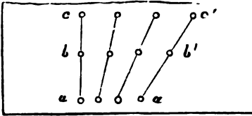
FIG. 3.— a, b, c, are stakes driven in the vertical wall of the side of a glacier; a', b', c', are the points occupied at a subsequent date.
