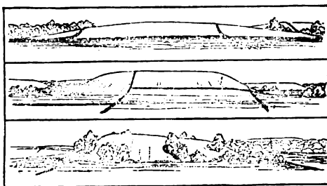
FIG. 78.—Outline of parallel drift-hills, in central New York. (Davis.)
