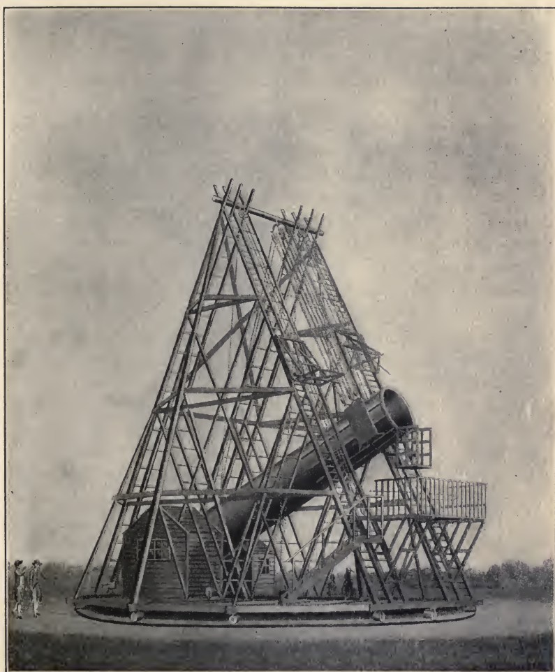
FIGURE 18. — Herschel's Telescope.
