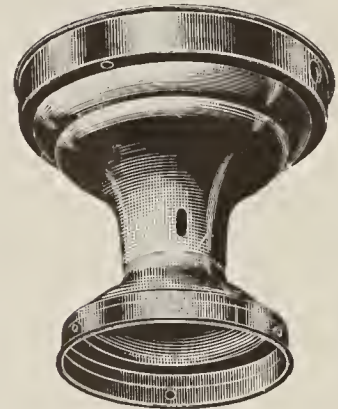
No. 1470 - 4" Fitter. Diameter 6" - Depth 5 1/4" No. 1468 - 2 1/4" Fitter. Diameter 6" - Depth 5" No. 1469 - 3 1/4" Fitter. Diameter 6" - Depth 5"
