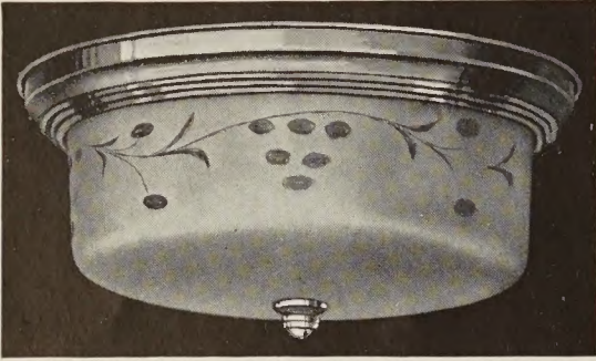
No. 159 - 1 Light. Diameter 7 \frac{5}{8} " - Depth 3 \frac{5}{8} " No. 160 - 2 Light. Diameter 8 \frac{3}{4} " - Depth 3 \frac{1}{2} " No. 161 - 2 Light. Diameter 11" - Depth 4" No. 162 - 3 Light. Diameter 13 \frac{1}{4} " - Depth 5" No. 163 - 4 Light. Diameter 15 \frac{1}{2} " - Depth 6 \frac{1}{2} "
