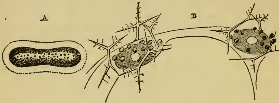
FIG. 5.— Sphærozoum punctatum .— A , a mass of the natural size; B , two of the oval central sacs with the colored vesicles and spicula which lie in the investing protoplasm, magnified.
