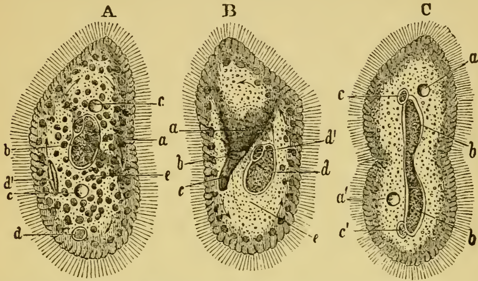
FIG. 10.— Paramœcium bursaria (after Stein).—A, the animal viewed from the dorsal side: a , cortical layer of the body; b , endoplast; c , contractile space; d d' , matters taken in as food; e , chlorophyll granules. B, the animal viewed from the ventral side: a , depression leading to b , mouth; c , gullet; d , endoplast; d' , endoplastule; e , central protoplasm. In both these figures the arrows indicate the direction of the circulation. C, Paramœcium dividing transversely: a a' , contractile spaces; b b' , endoplast dividing; c c' , endoplastules.
