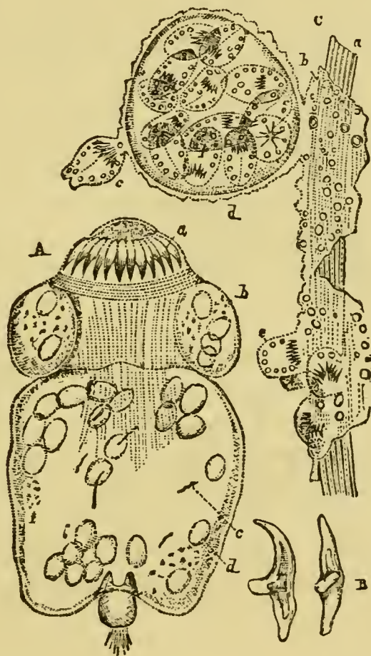
FIG. 48.-- Echinococcus veterinorum .—A, "Tænia head," or Scolex : a, hooks; b, suckers; c, cilia in water-vessels; d, oval, strongly refracting particles; B, single hooks; C, portion of the elastic cyst, a; with the inner membranous primary cyst, b; c and e, Scolices developing from its inner surface; d, a secondary cyst.
