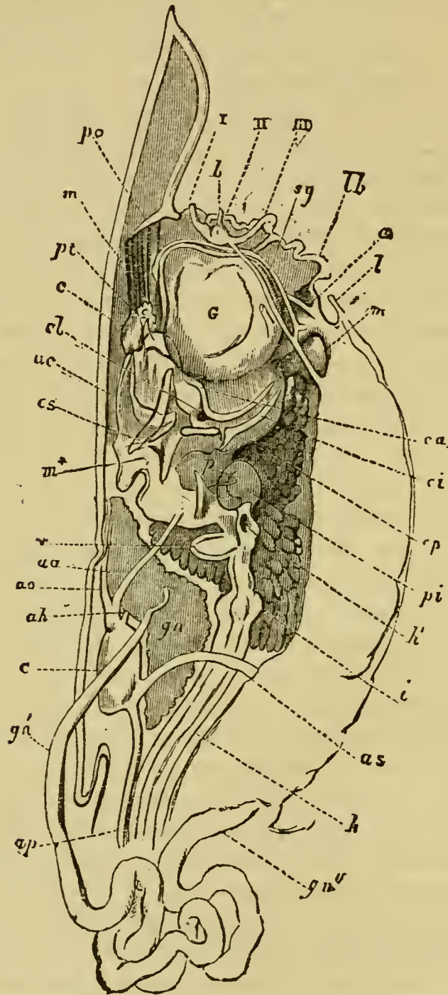
FIG. 74.— Astacus , Longitudinal Section.—I, II, III, Sterna of first, second, and third somites; a , oesophagus; lb , labrum; l , metastoma; G , membranous part of the stomach; c , cardiac ossicle; pt , pterocardiac; uc , urocardiac; cl , lateral cardiac; p , cardio-pyloric valve; pi , inferior pyloric valvular apparatus; m , anterior gastric muscle; m* , insertion of posterior gastric muscles; pc , procephalic processes; h' , opening of hepatic duct; v , pyloric caecum; i, k , intestine; gn , testis; gn', gn'' , vas deferens; C , heart; ao , ophthalmic artery; aa , antennary; ah , hepatic; as , sternal; ap , superior abdominal artery; b , cerebral ganglia; sg , azygos visceral nerve.
