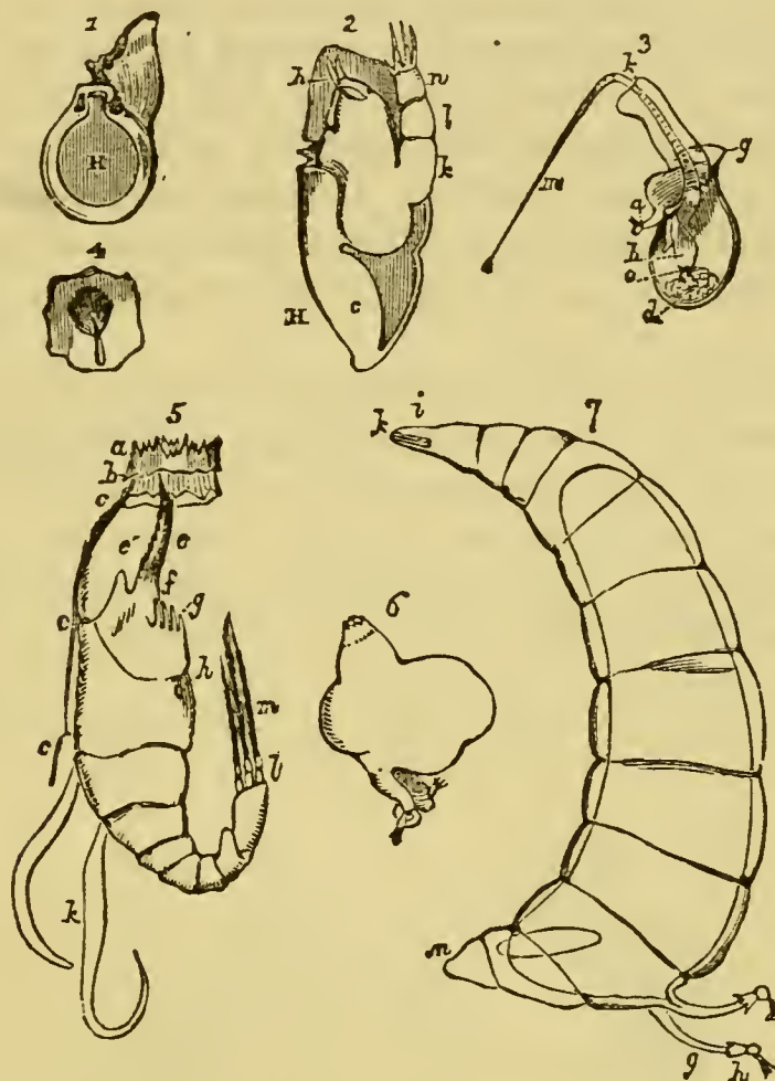
FIG. 69.—1. Alciippe lampas ; female. 2. The same in sectional view: H , Horny disk of attachment; in 1, the males are visible as dark specks on either side of the upper part of the sac; c , ovary; h , first pair of cirri; k , l , n , three segments of the thorax without cirri; the other three segments, bearing the three pairs of terminal cirri, are very short. 3. Male Alciippe : a , antennary appendages; b , vesicula seminalis; o , eye; d , testis; k , orifice of the sac; m , penis. 4. Burrow of Alciippe in a portion of a Fusus shell. 5. Cryptophialus minutus (female) with the outer integument removed: e , labrum; f , palpi; g , outer maxillæ; h , rudimentary maxillipede; c , wall of sac continued above into the rim of the aperture a . b ; l , m , abdominal cirri; k , appendages of unknown nature. 6. Male Cryptophialus . 7. Proteolepas bivincta ; m , mouth; g , h , peduncle and antenna; i , k , vesicula seminalis and penis. (After Darwin.)
