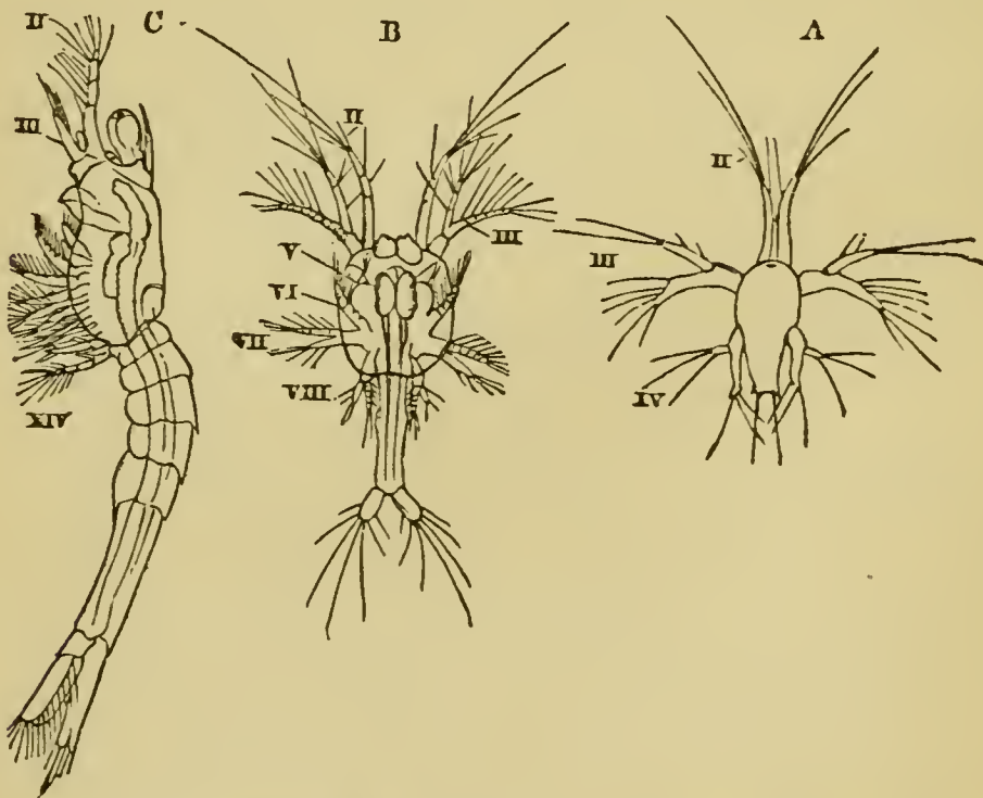
FIG. 77.— Peneus .—A, Nauplius-stage. B, Zoëa or Copepod stage. C, Schizopod-stage. (After Müller.)
