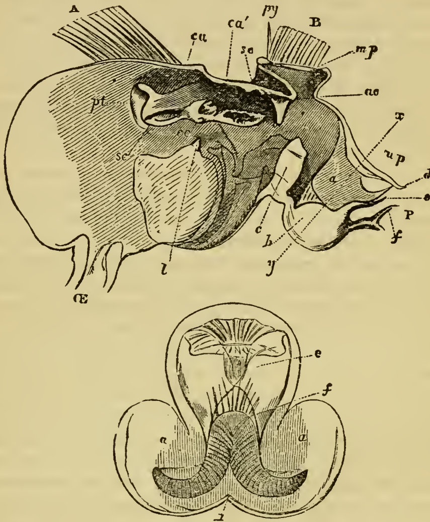
FIG. 73.— Astacus .—Upper Figure: Longitudinal Section of Stomach.—A, anterior gastric muscle; B, posterior gastric muscle; E, œsophagus; P, pylorus; ca, cardiac ossicle; ca', its urocardiac process; ac, urocardiac tooth; py, pyloric ossicle; the oblique bar, extending from the end of the cardiac to the pyloric, is the pre-pyloric ossicle; pt, pterocardiac; se, postero-lateral cardiac, with its great tooth, cc; l, small inferior tooth; c, cardio-pyloric valve; b, infero-median pyloric ridge; a, lateral pyloric ridge; d, superior pyloric ridge; up, uro-pyloric ossicle; x y, line of section; the anterior face of the posterior segment being shown in the lower figure.
