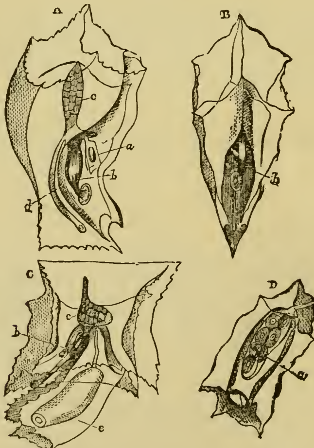
FIG. 23.— A , B , Diphyzoïd ( Sphenoides ), lateral and front views. C , Diphyzoïd of Abyla ( Cuboïdes ). a , e , gonophore or reproductive organ; b , hydranth; c , phyllocyst or cavity of hydrophyllium, with its process ( d ). D , free gonophore, its manubrium ( a ) containing ova.
