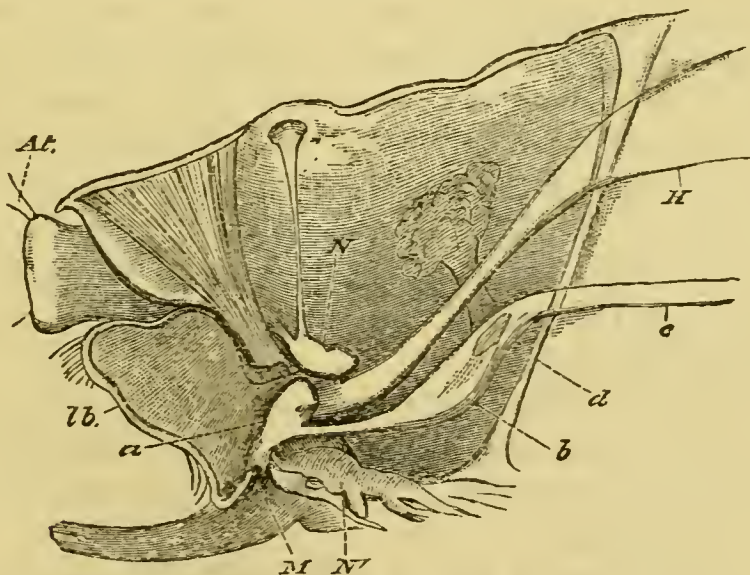
FIG. 86.— Scorpio .—Vertical section of the cephalo-thorax: At. , chelicera; lb. , labrum; M , mouth; a , pharyngeal sac; N , N' , supra and infra-oesophageal ganglia; b , œsophagus; d , opening of the salivary ducts; e , intestine; H , heart.
