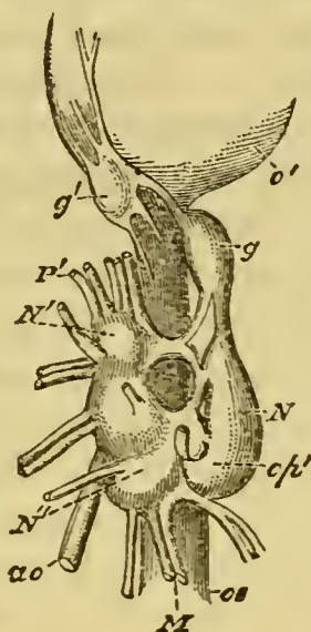
FIG. 123.— Sepia officinalis .—The nervous mass which surrounds the gullet; N , the cerebral; N'' , the pedal; N''' , the parieto-splanchnic ganglion; ao , the aorta; oe , the œsophagus; o'' , buccal nerves; P'' , nerves to the anus; M , pallial nerves; g , superior; g'' , inferior buccal ganglion. (After Garner.) 1
