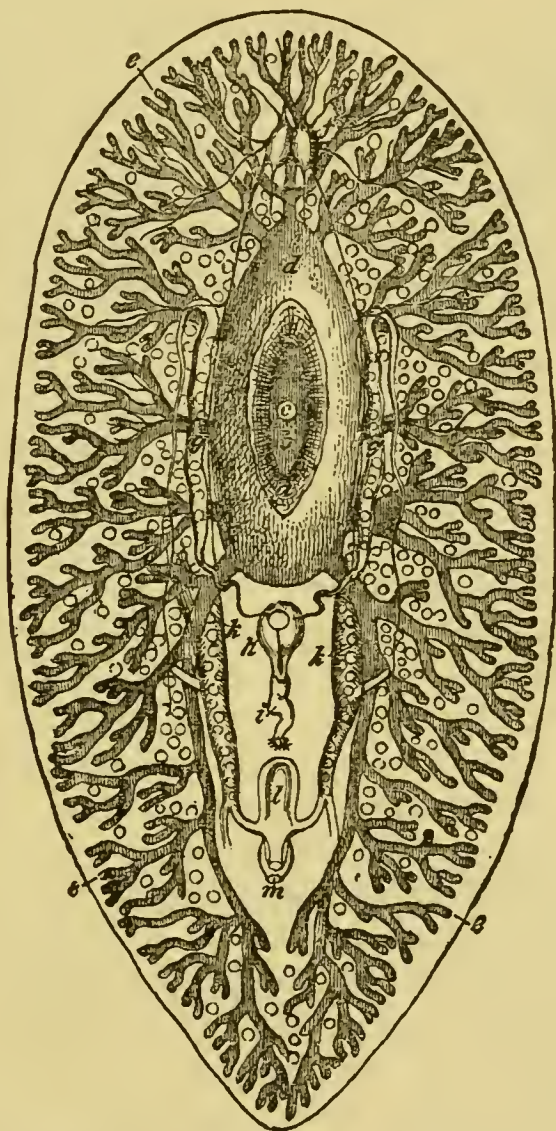
FIG. 33.— Polycelis (Leptoplana) lævigata (after Quatrefages).— a , mouth; b , buccal cavity; c , œsophageal orifice; d , stomach; e , ramifications of gastric cœca; f , ganglia; g , testes; h , vesiculæ seminales; i , male genital canal and penis; k , oviducts; l , spermathecal dilatation at their junction; m , vulva.
