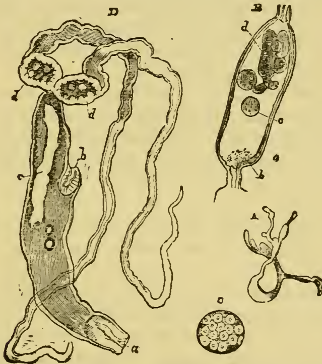
FIG. 45.— Bucephalus polymorphus of the fresh-water muscle.—A, ramified sporocyst ; B, portion of the same more magnified: a, outer coat, b, inner ; c, d, germ-masses in course of development ; C, one of the germ-masses more highly magnified ; D, Bucephalus : a, b, suckers ; c, clear cavity ; d, caudal appendages.
