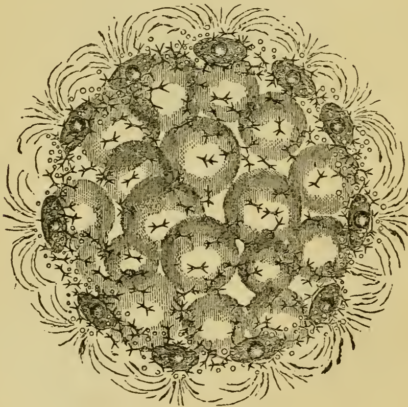
FIG. 6.— Sphærozoum ovodimare (after Haeckel), magnified.
