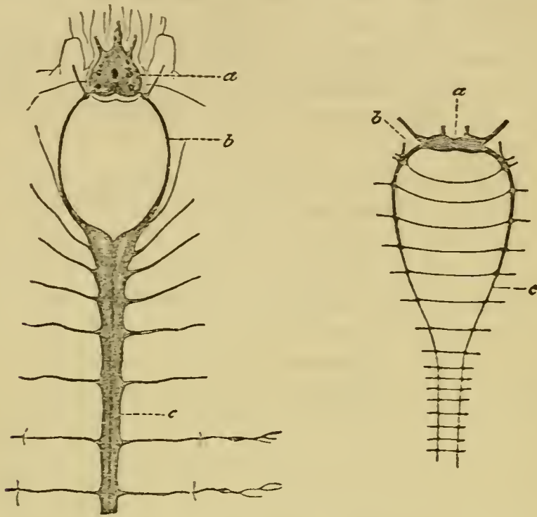
FIG. 55.—A, anterior end of the nervous system of Polydora squamata (after De Quatrefages): a , cerebral ganglia; b , œsophageal commissures; c , longitudinal commissures of the ventral ganglia. B, anterior end of the nervous system of Sabella fiabellata (after De Quatrefages): a , cerebral ganglia; b , œsophageal commissures; c , longitudinal commissures of the ventral ganglia. Those of opposite sides are united by long transverse commissures.
