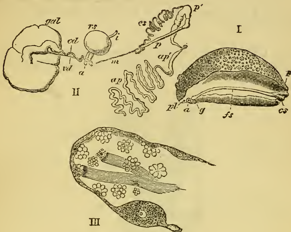
FIG. 123.—I. Peronia verruculata .— a , anus; pl , pulmonary aperture; g , genital aperture; fs , seminal groove; p , opening for the penis. II. Generative organs of the same animal, the ovotestis being omitted.— gal , gland which furnishes a glairy secretion; od , oviduct; vd , vas deferens; i , intestine; a , anus; rs , receptaculum seminis; p , aperture of the penis; p' , penis; cs , seminal duct; ap , glandular appendage; m , retractor muscle of the penis. (After Keferstein.) III. Blind end of a follicle of the ovotestis of Helix pomatia . At the apex the spermatozoa are seen in different stages of development, the fully-formed spermatozoa floating in bundles in the cavity of the follicle. Lower down, ova are developing in the walls of the follicle. (After Keferstein and Ehlers.)
