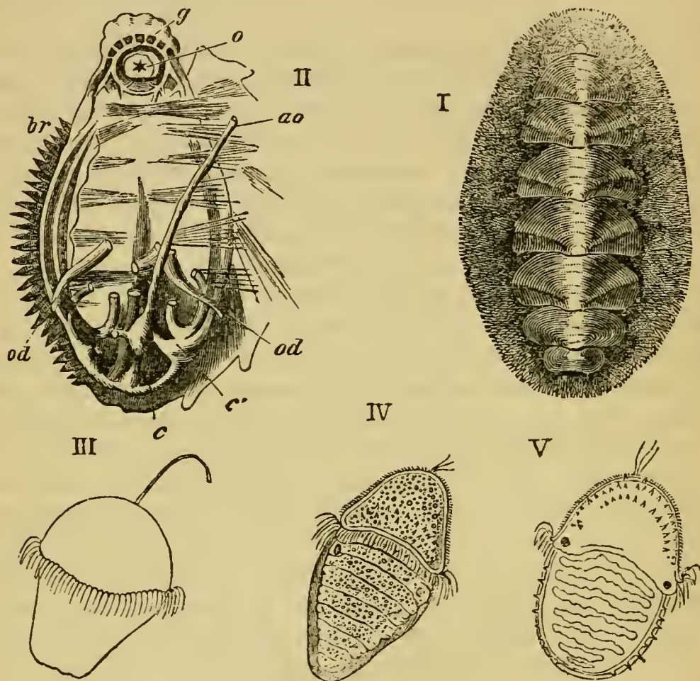
FIG. 121.—I. Chiton Wossnessenskii . (After Middendorf.) II. Chiton dissected to show o , the mouth; g , the nervous ring; ao , the aorta; c , the ventricle; c' , an auricle; br , the left branchiæ; od , the oviducts. (After Cuvier.) III, IV., V. Stages of development of Chiton cinereus . (After Lovén.)
