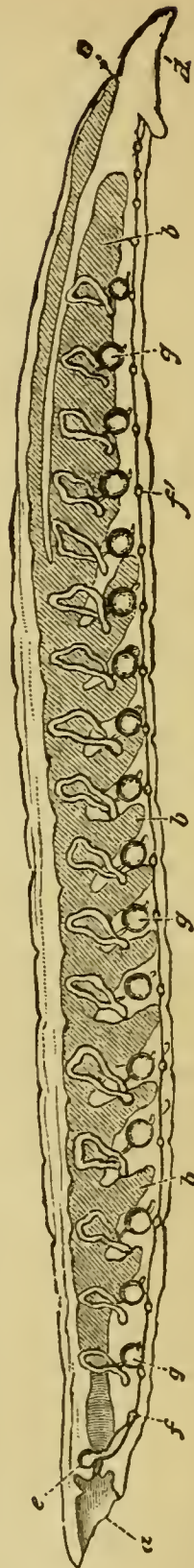
FIG. 49.—A longitudinal and vertical section of the body of the Leech ( Hirudo medicinalis ), after Leuckart. 1 — a , the mouth; b, b' , sacculations of the alimentary canal; c , the anus; d , the terminal sucker; e , the cerebral ganglia; f, f' , the chain of post-oesophageal ganglia; g, g, g' , the segmental organs.
