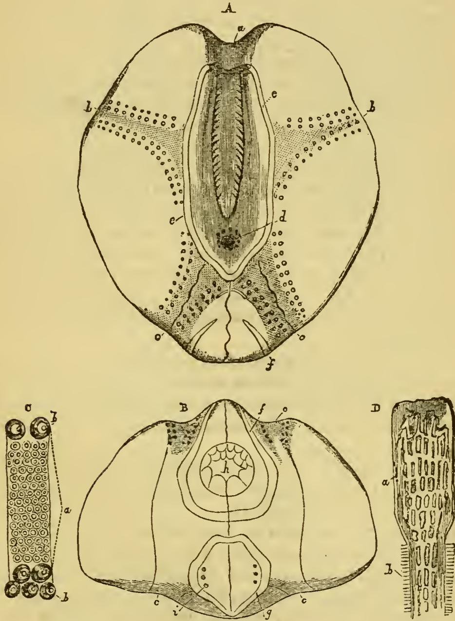
FIG. 143.— Amphidotus cordatus .—A, viewed from above; B, from behind: a, b b , trivium, or anterior and anterolateral ambulacra; c c , bivium, or posterolateral ambulacra; d , madreporic tubercle, surrounded by the genital apertures; e , intrapetalous semita ; f , circumanal semita ; g , subanal semita ; h , anus; i , intrasemital pores of bivial ambulacra. C, semita magnified: a , semital tubercles; b , ordinary tubercles. D, semital spine : a , terminal enlarged, non-ciliated portion; b , ciliated stem.
