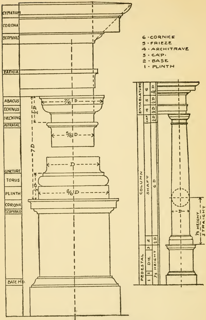
Fig. 83. The Tuscan Order.
