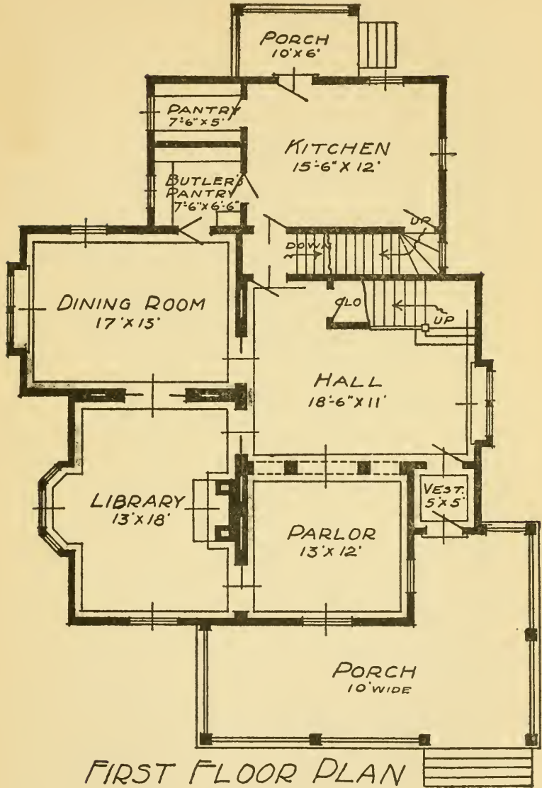
Fig. 4. Final Preliminary Drawing. Drawn with T-square and triangles to scale.
