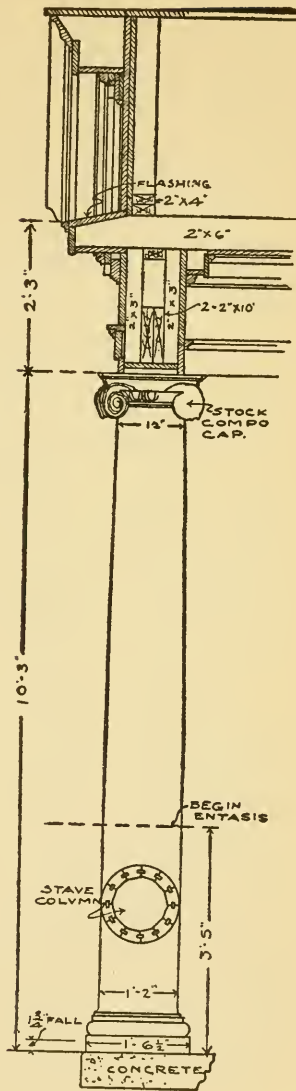
Fig. 23. Porch of Fig. 21 Detailed for Wood Construction.
