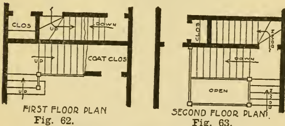
Fig. 62. Combination Front and Back Stairs. Fig. 63.
