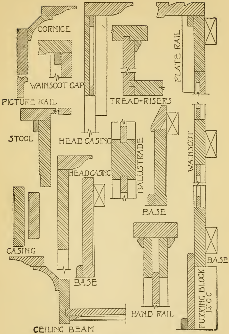
Fig. 16. A Sheet of Full-Sized Details
