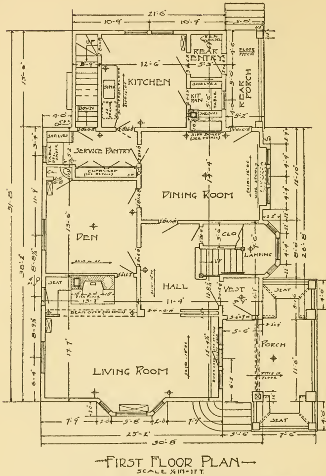
Fig. 9. First-Floor Plan of a Residence at Champaign, Ill. The scale reproduced is valid only as referring to the original-sized drawing.
