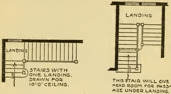
Fig. 60. Types of Stairs with One Landing. Fig. 61.
