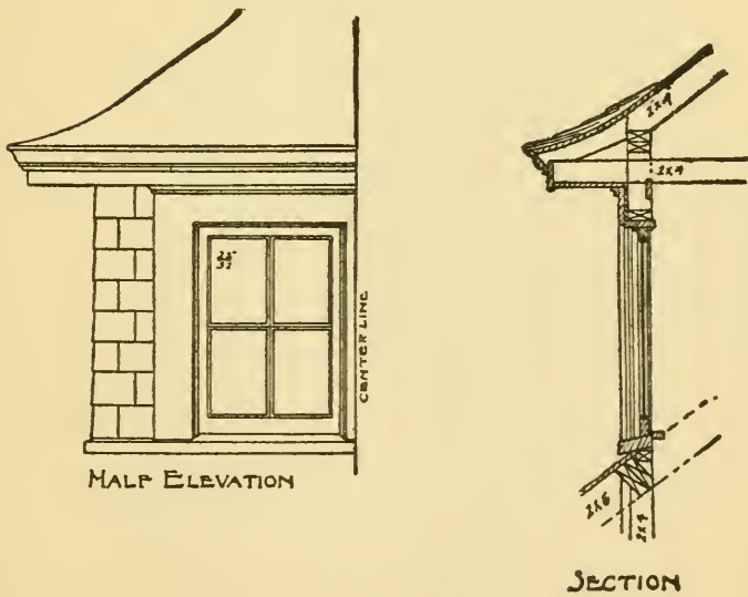
Fig. 74. Details for a Dormer or Roof Window.
