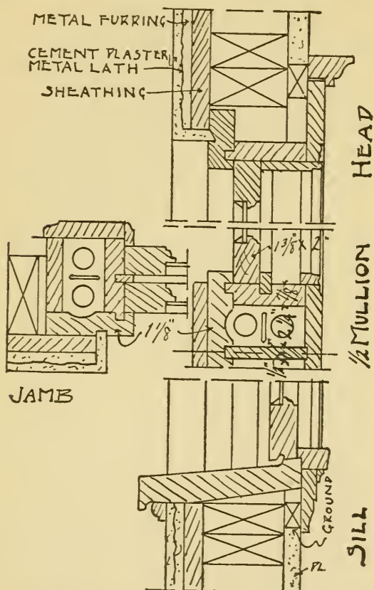
Fig. 71. Double-Hung Window, Outside of Building Plastered.
