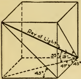
Fig. 26. Drawing Showing Assumed Direction of Light.
