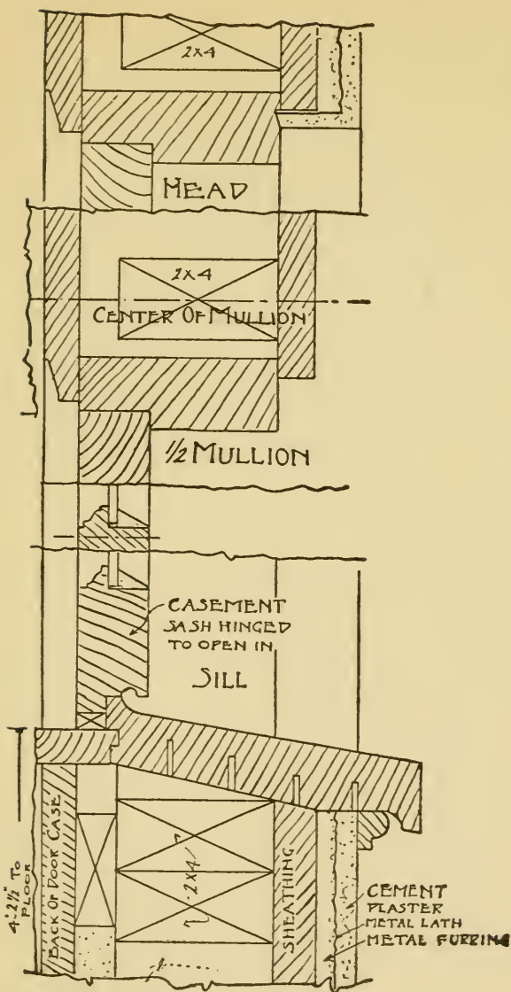
Fig. 76. Details of Casement Window.
